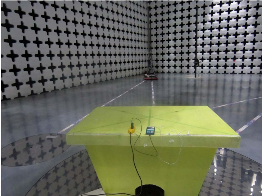
Charger RE below 1GHz
