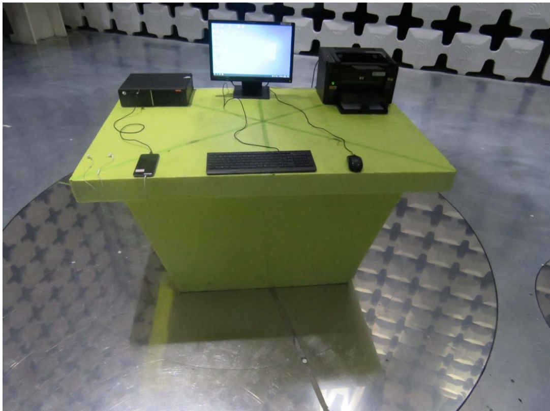
USB RE below 1GHz
