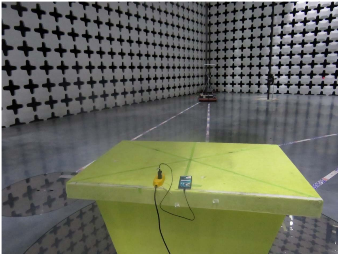
RE below 1GHz
