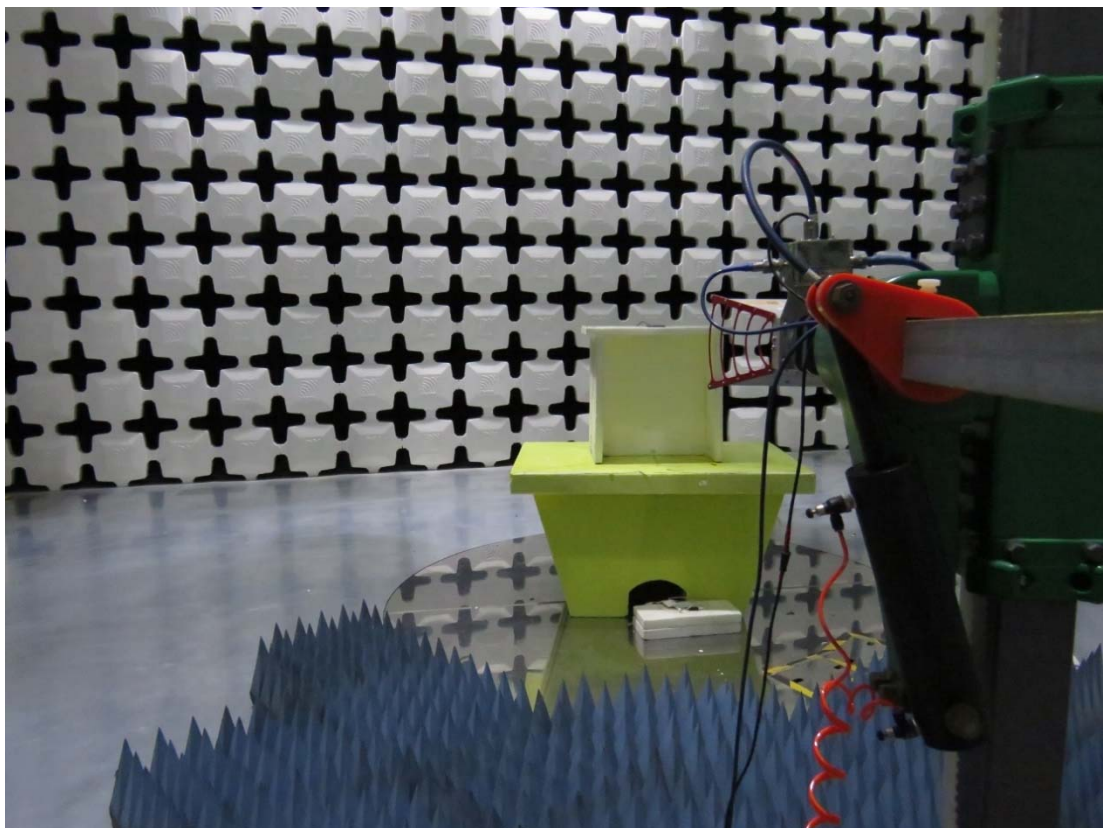
RE above 1GHz
