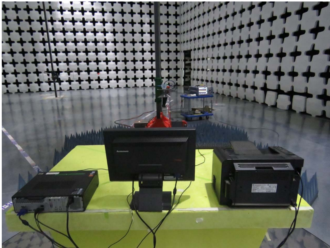
USB RE above 1GHz
