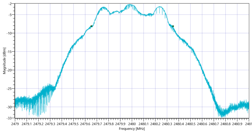
Plot_FCC Part 15.247 Maximum Peak Conducted Output Power DTS ~ BT LE 1 Msps DTS BW_22032021_112426.png
