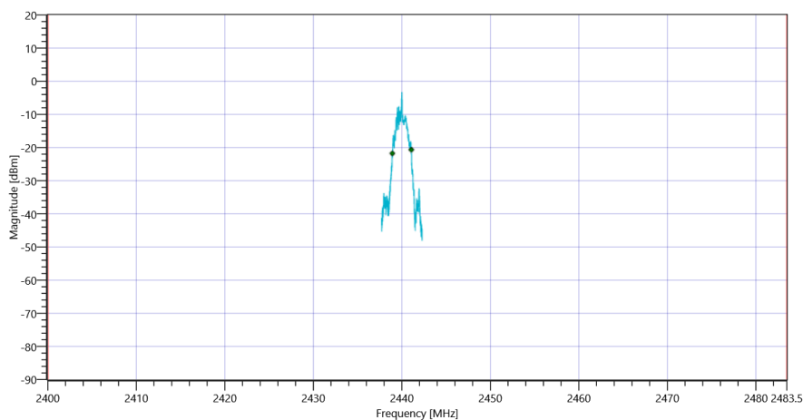
Plot_FCC Part 15.247 Bandwidth 99PCT-20dB ~ BT LE 2 Msps 22032021_120229.png
