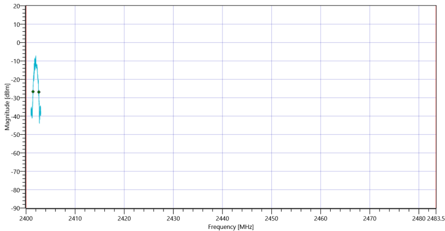
Plot_FCC Part 15.247 Bandwidth 99PCT-20dB ~ BT LE 1 Msps 22032021_110242.png
