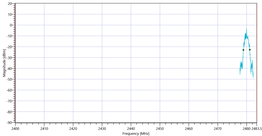
Plot_FCC Part 15.247 Bandwidth 99PCT-20dB ~ BT LE 2 Msps 20dB_22032021_123505.png
