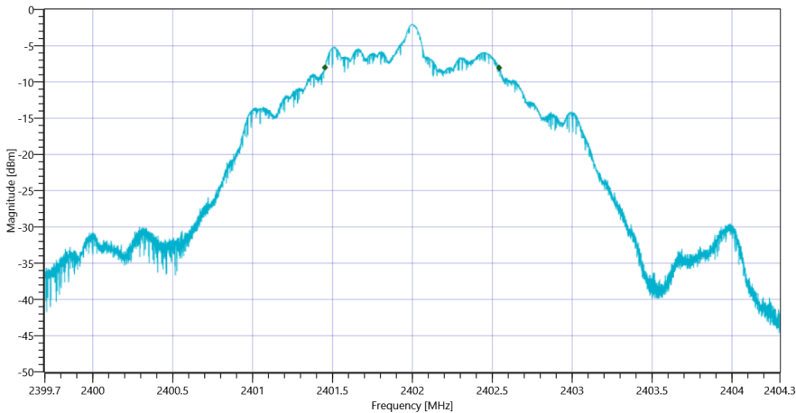
Plot_FCC Part 15.247 Bandwidth 6dB DTS ~ BT LE 2 Msps_22032021_113558.png
