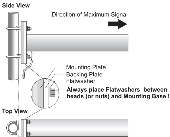
Figure 4-1 Mounting the 14 dBi Antenna to a Mast
