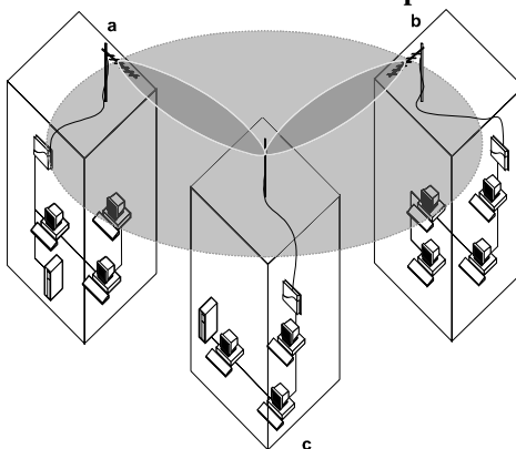
Figure 1-2 WaveCAMPUS Point-to-Multipoint Link
