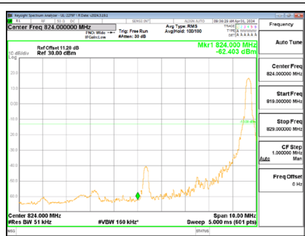
LTE5 5MHz 16QAM LOW Ch RB1-24
