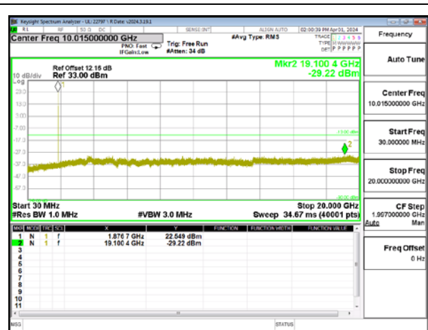
LTE25 15MHz 16QAM MID Ch RB1-0
