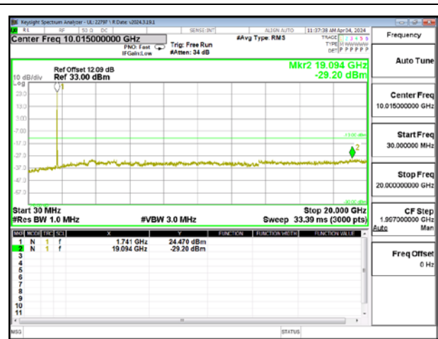
LTE66 15MHz 16QAM MID Ch RB1-0
