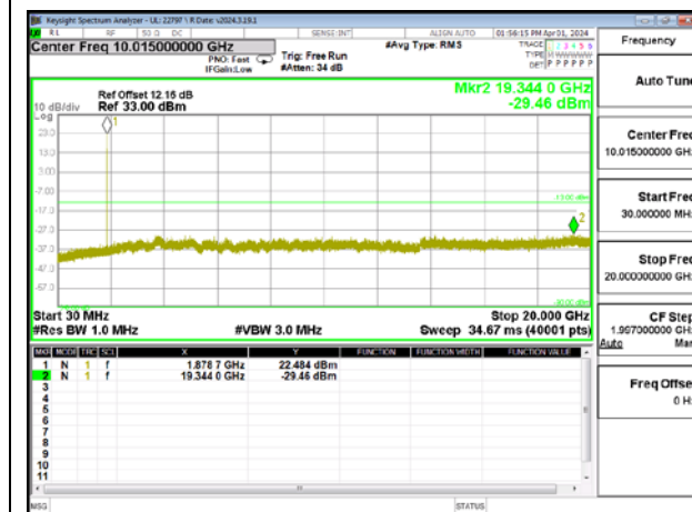
LTE25 10MHz 16QAM MID Ch RB1-0
