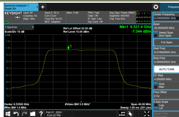
Channel 117 (6535MHz)
