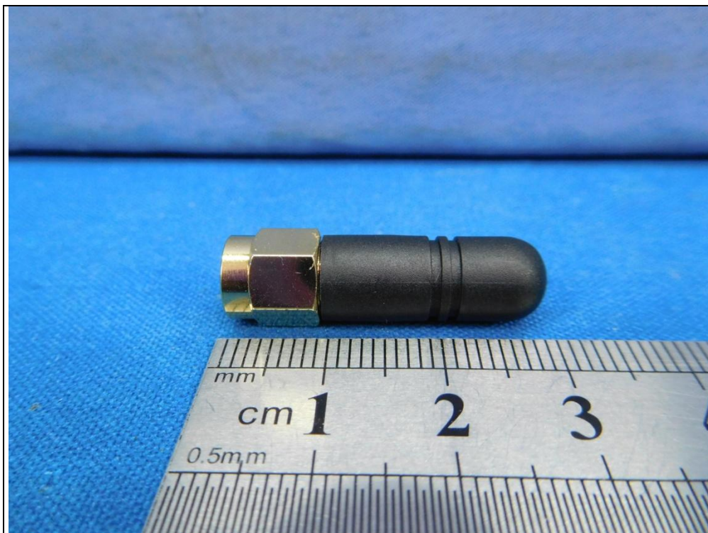
Antenna 1
