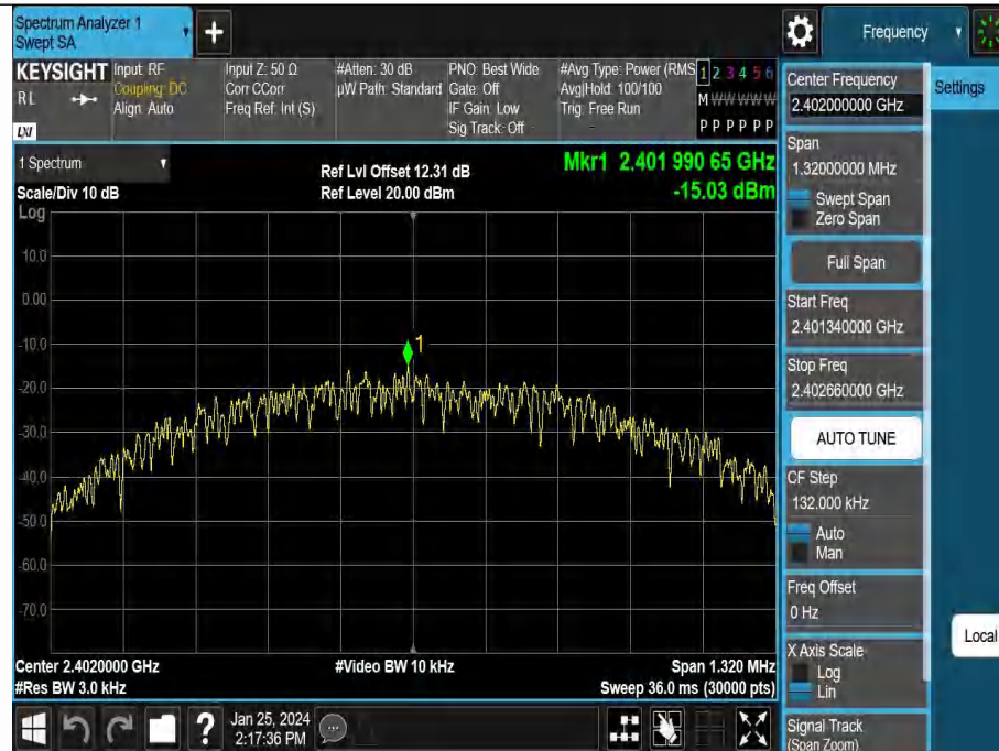
BLE_1M-Ant1-2402-PASS
