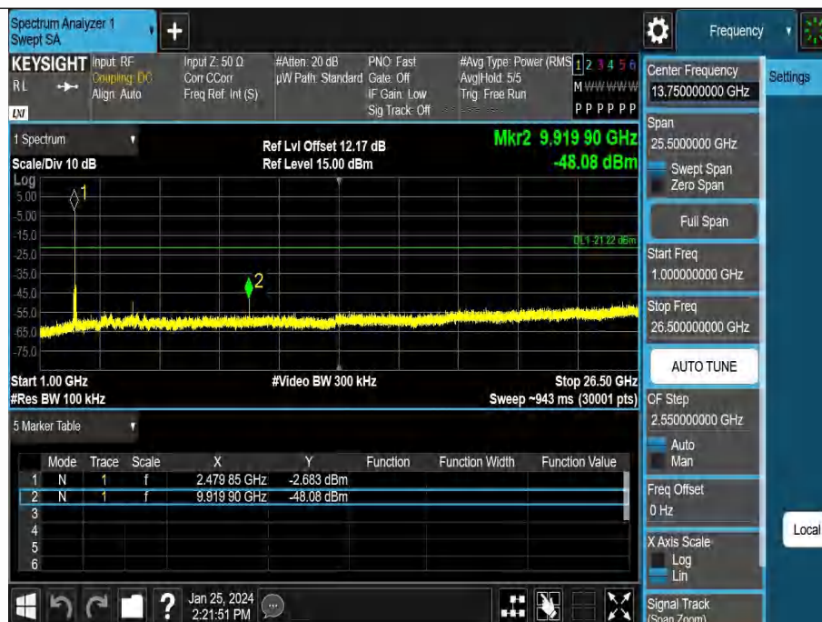
BLE_1M-Ant1-2480-1000~26500-PASS
