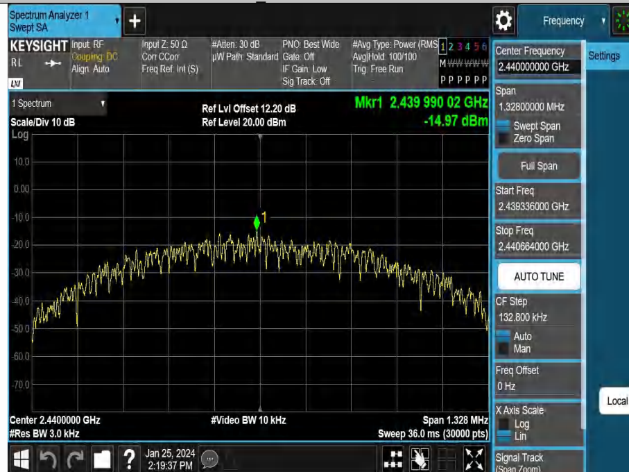
BLE_1M-Ant1-2440-PASS
