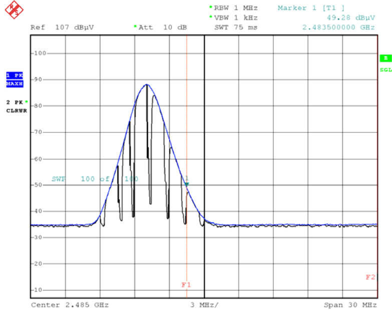
Radiated Restricted Band Edges plot – Average Reading ( \pi/4 DQPSK, Ch.78)
