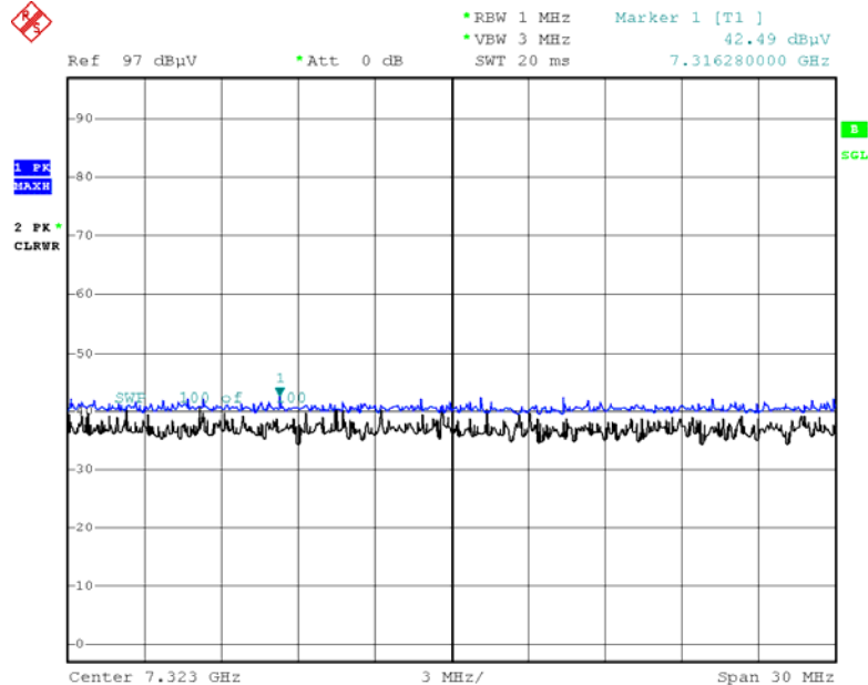
Radiated Spurious Emissions plot – Peak Reading ( \pi /4QPSK, Ch.39 3rd Harmonic)
