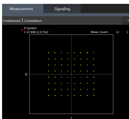
64QAM
