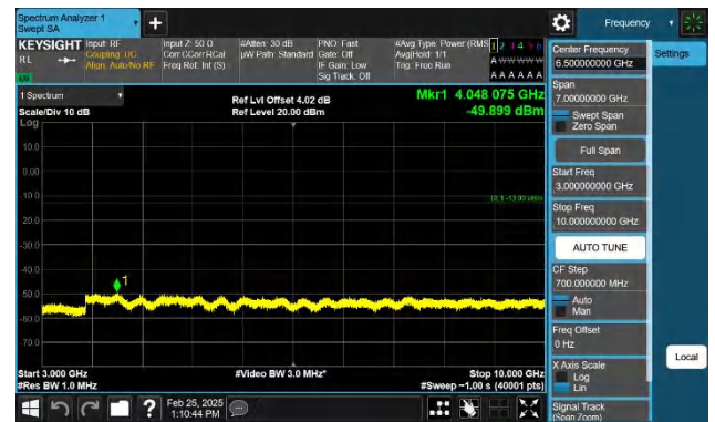
Band13-10MHz-QPSK-23230-1RB#49-3000~10000-PASS
