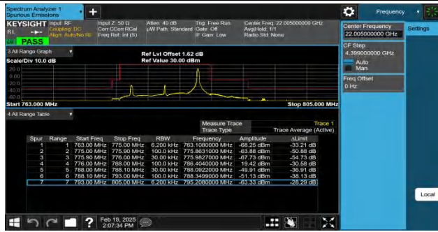
Band13-10MHz-QPSK-23230-1RB#49-PASS
