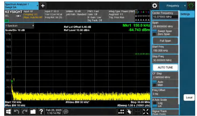
Band13-10MHz-QPSK-23230-1RB#49-0.15~30-PASS
