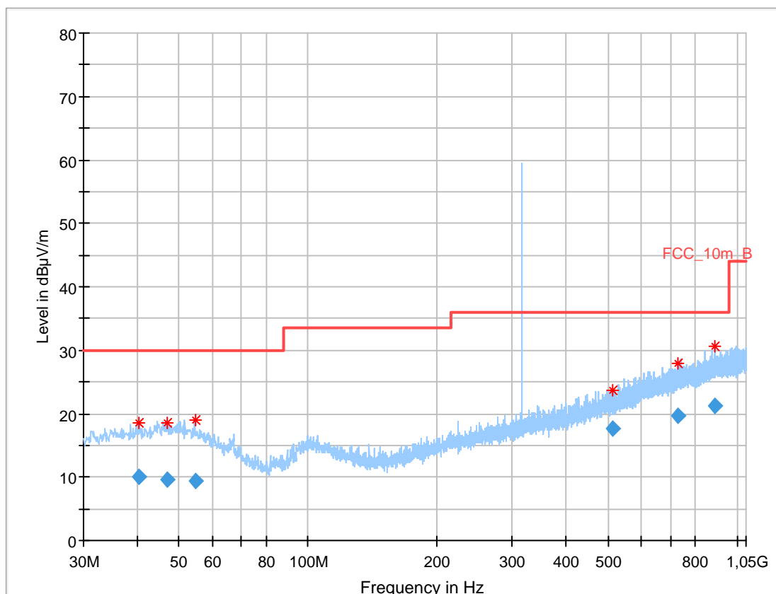
Plot 2: 30 MHz to 1000 MHz, vertical & horizontal polarisation
