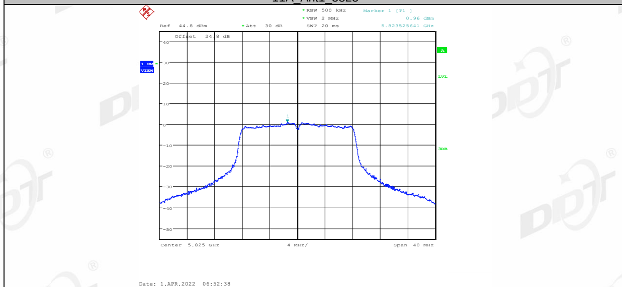
11A Ant2 5825
