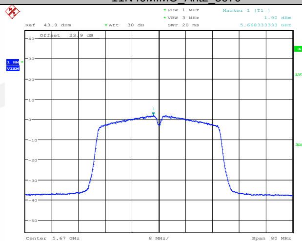
11N40MIMO Ant2 5670
