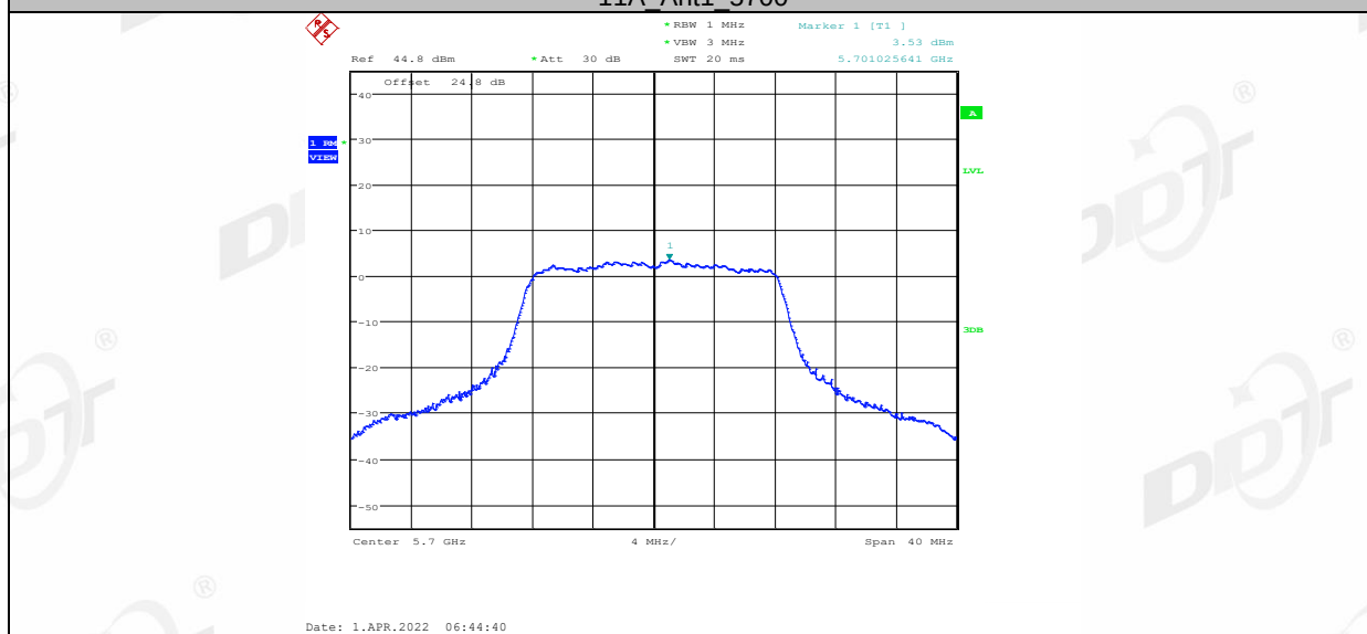
11A Ant2 5700
