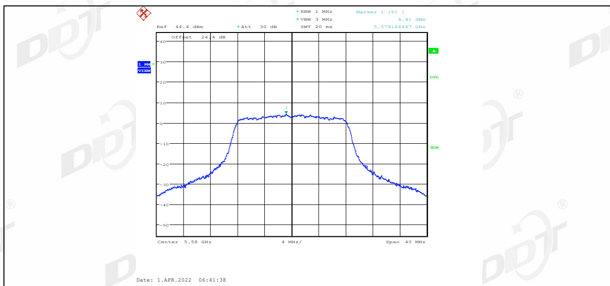
11A Ant2 5580
