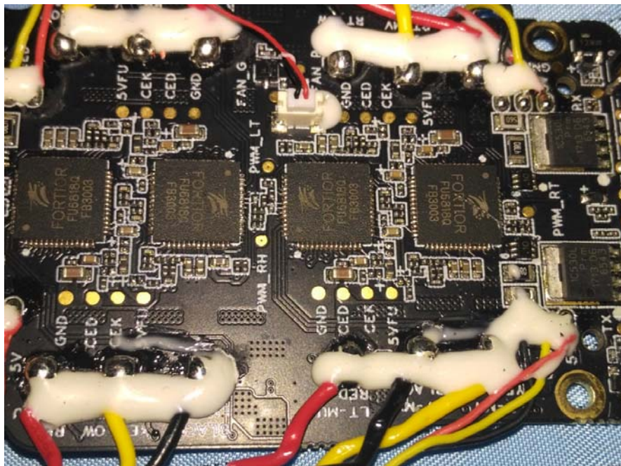
EUT – Main Board 1 Main Chip View
