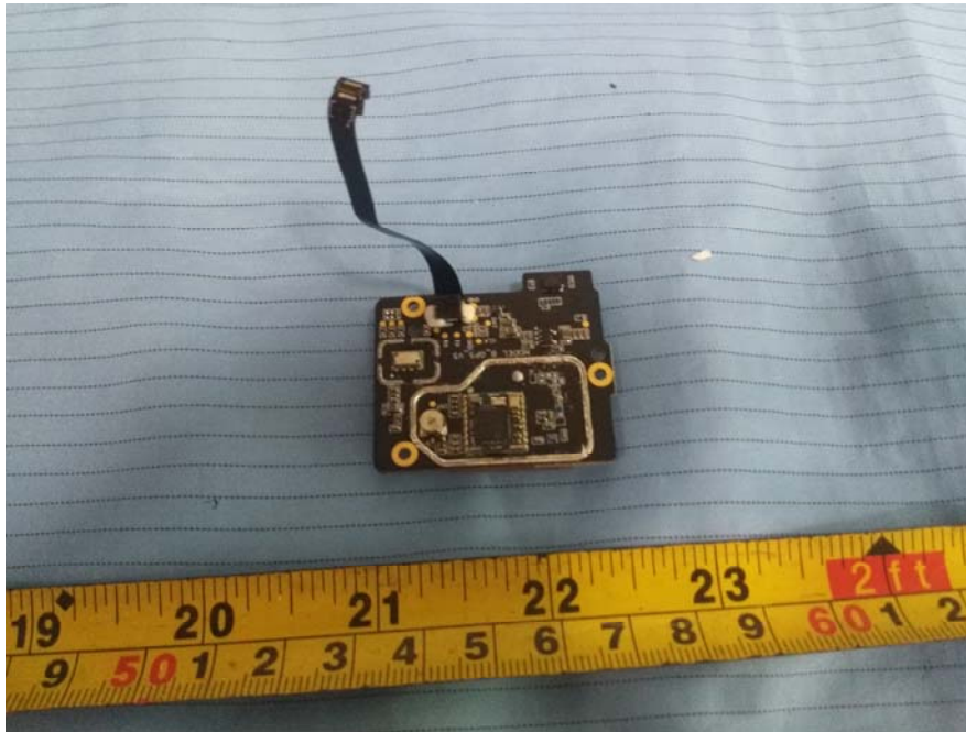
EUT – GPS Board Top Shielding off View 2
