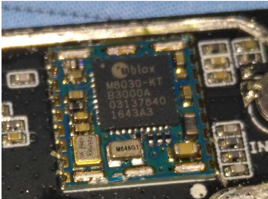
EUT – GPS Board Main Chip View
