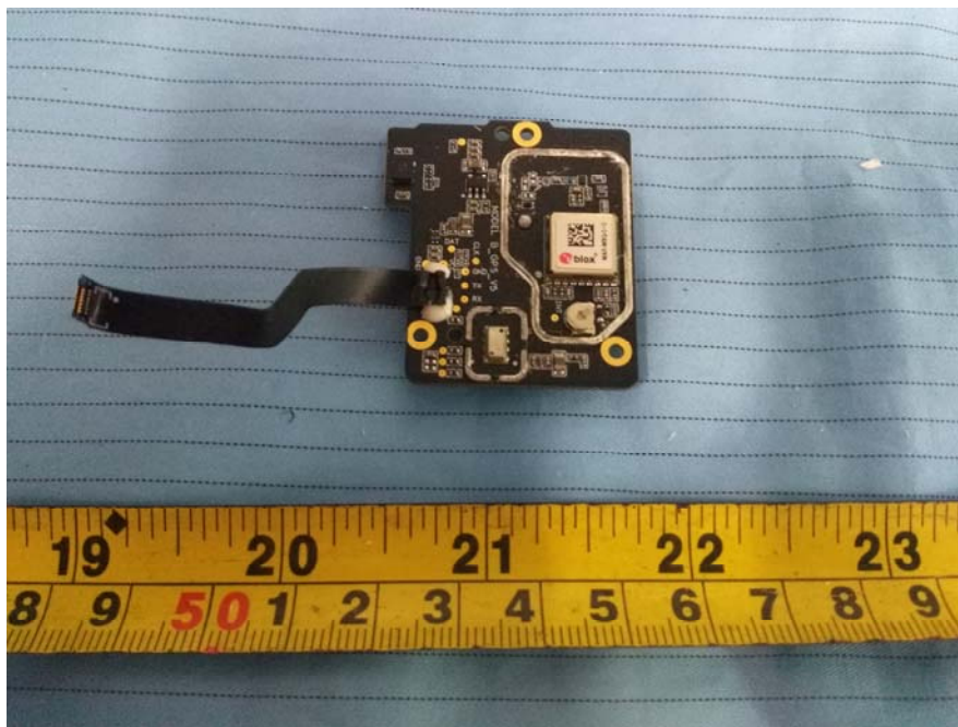
EUT – GPS Board Top Shielding off View 1
