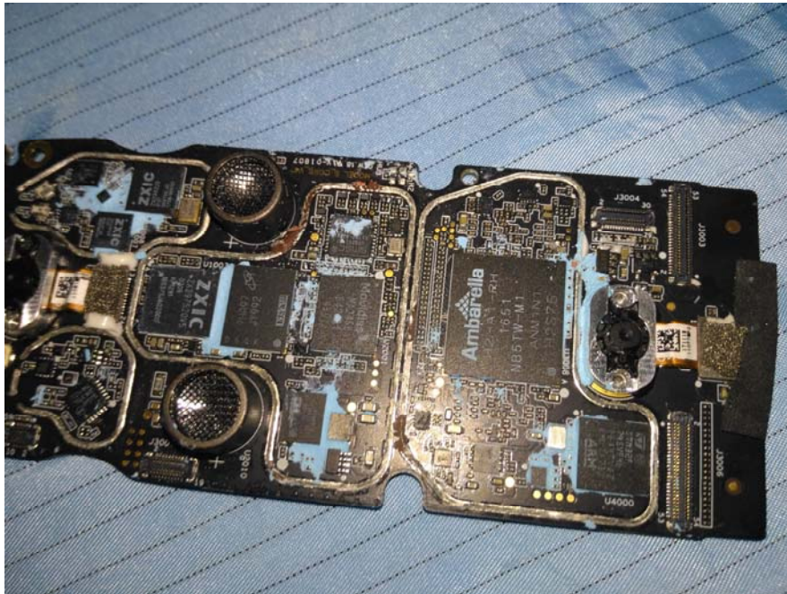
EUT – Main Board 3 Top Main Chip View
