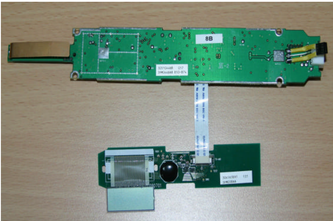
Solder View of PCB 1
