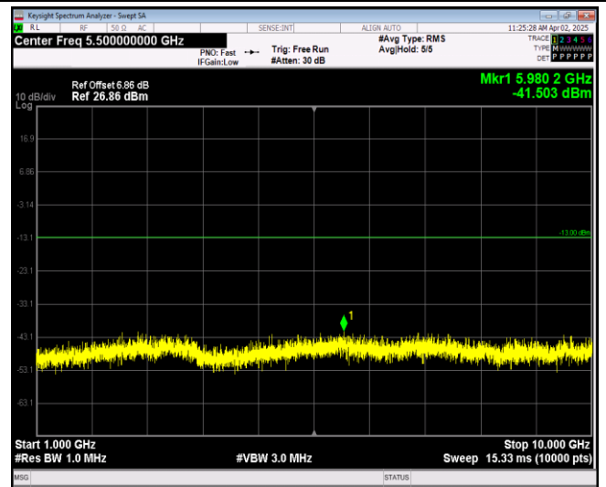
Band17-10MHz-16QAM-23800-1RB#0-Range2:1000~10000MHz
