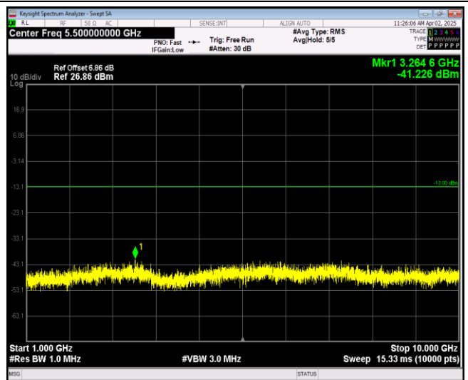
Band17-10MHz-16QAM-23780-1RB#0-Range2:1000~10000MHz
