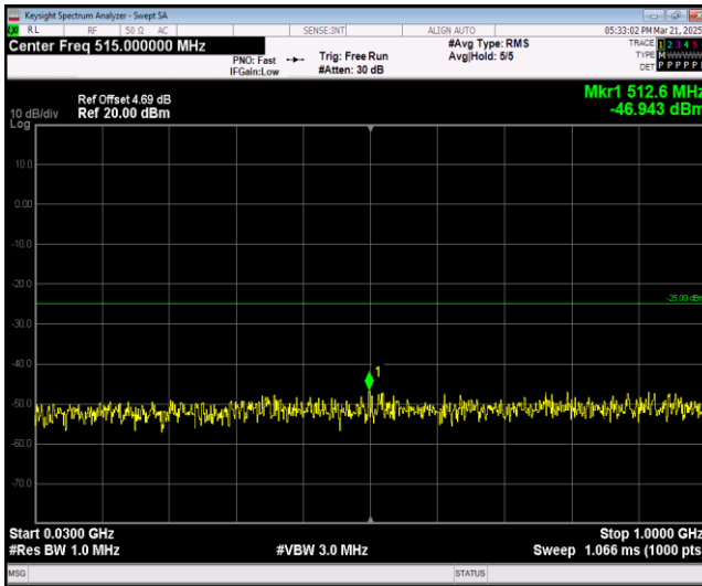
Band38-5MHz-16QAM-37775-1RB#0-Range1:30~10 00MHz
