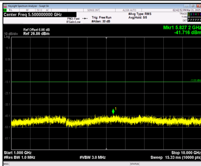
Band17-5MHz-QPSK-23825-1RB#0-Range2:1000~1 0000MHz
