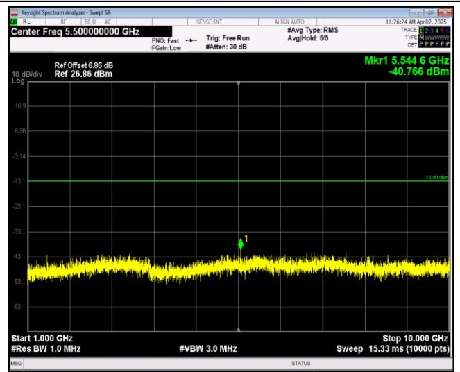
Band17-10MHz-16QAM-23800-1RB#0-Range2:1000~10000MHz
