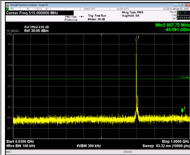
Band17-10MHz-16QAM-23800-1RB#0-Range1:30~1000MHz
