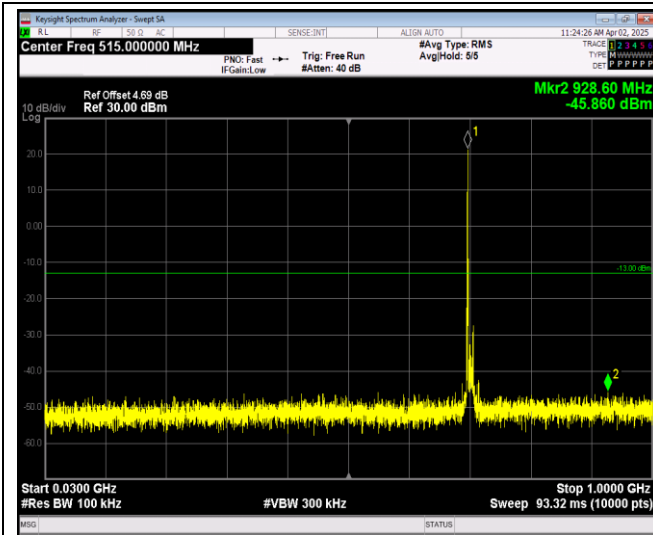
Band17-10MHz-16QAM-23790-1RB#0-Range1:30~1000MHz
