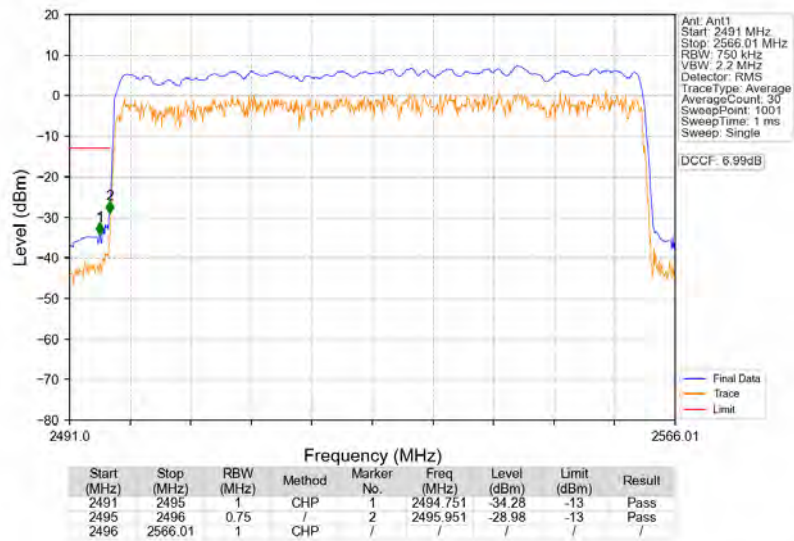
n41_30kHz_SISO_NTNV_70MHz_DFT-s-OFDM_PI/2_BPSK_2531.01MHz_Outer_Full
