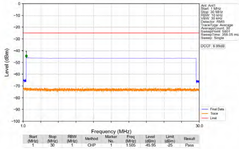
n41_30kHz_SISO_NTNV_50MHz_CP-OFDM_QPSK_2521.02MHz_Edge_1RB_Left
