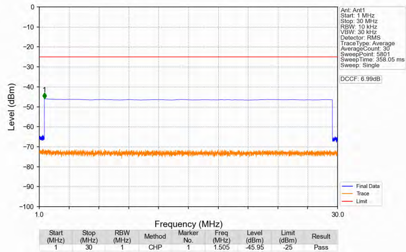
n41_30kHz_SISO_NTNV_70MHz_DFT-s-OFDM_QPSK_2592.99MHz_Edge_1RB_Left
