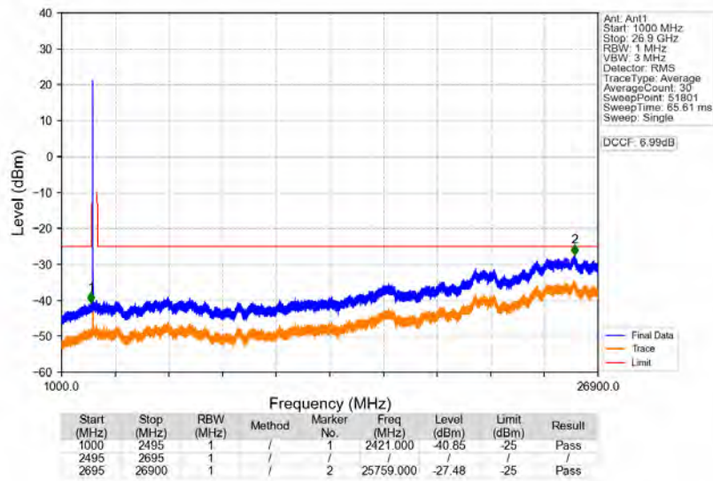
n41_30kHz_SISO_NTNV_50MHz_CP-OFDM_QPSK_2521.02MHz_Edge_1RB_Left
