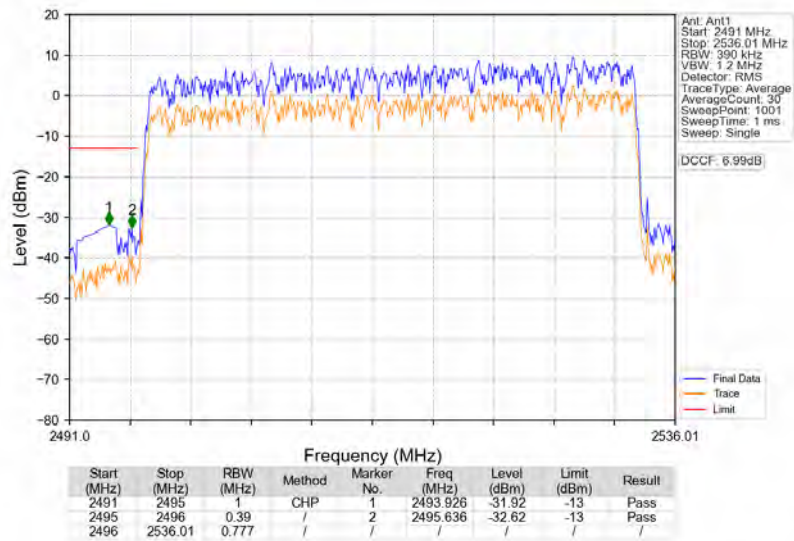
n41_30kHz_SISO_NTNV_40MHz_DFT-s-OFDM_QPSK_2516.01MHz_Outer_Full
