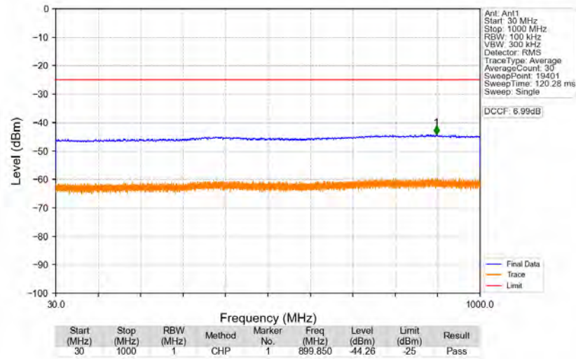
n41_30kHz_SISO_NTNV_50MHz_CP-OFDM_QPSK_2521.02MHz_Edge_1RB_Left
