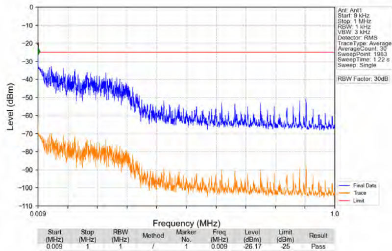
n41_30kHz_SISO_NTNV_60MHz_CP-OFDM_QPSK_2659.98MHz_Edge_1RB_Right
