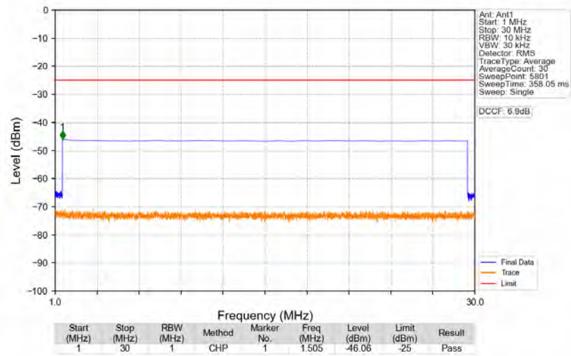
n41_30kHz_SISO_NTNV_50MHz_CP-OFDM_QPSK_2592.99MHz_Edge_1RB_Left
