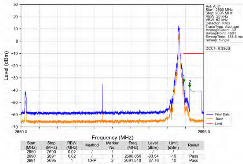
n41_30kHz_SISO_NTNV_40MHz_DFT-s-OFDM_PI/2_BPSK_2670MHz_Edge_1RB_Right
