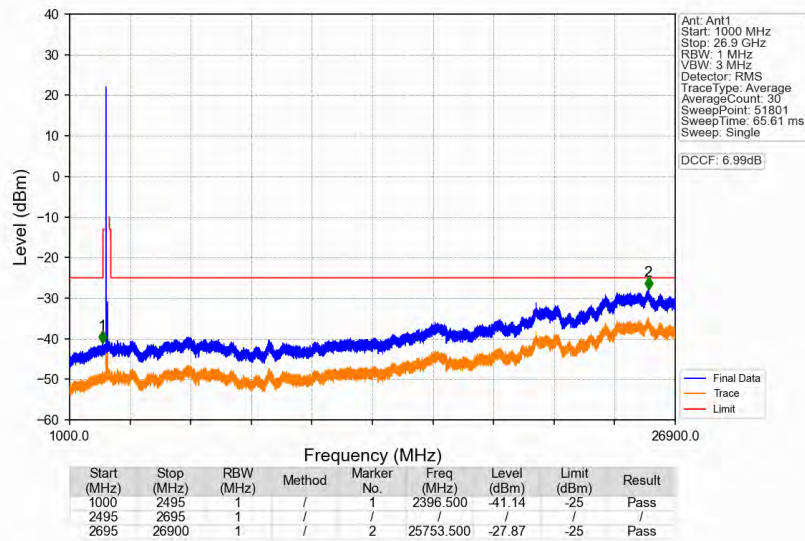
n41_30kHz_SISO_NTNV_70MHz_CP-OFDM_QPSK_2592.99MHz_Edge_1RB_Left
