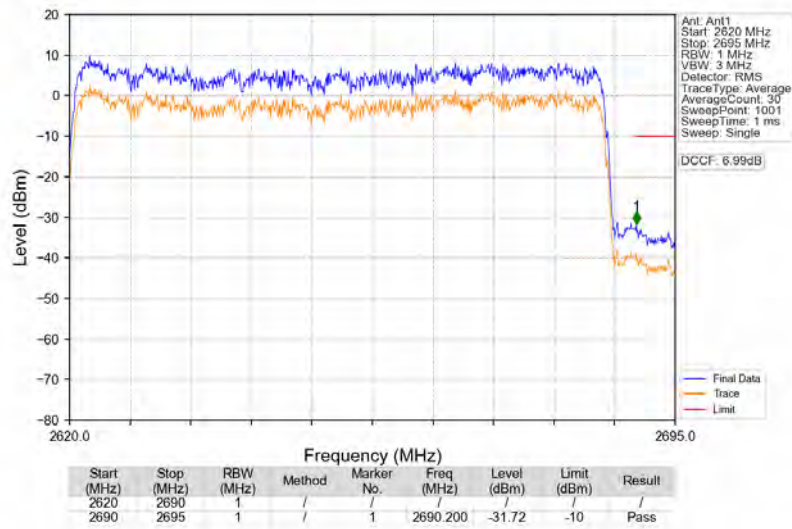
n41_30kHz_SISO_NTNV_70MHz_DFT-s-OFDM_PI/2_BPSK_2655MHz_Outer_Full
