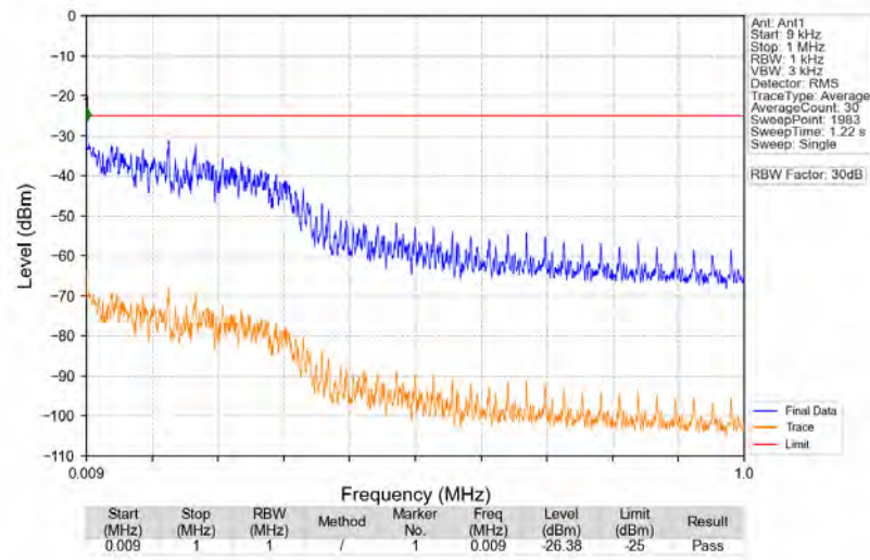
n41_30kHz_SISO_NTNV_50MHz_CP-OFDM_QPSK_2592.99MHz_Edge_1RB_Left
