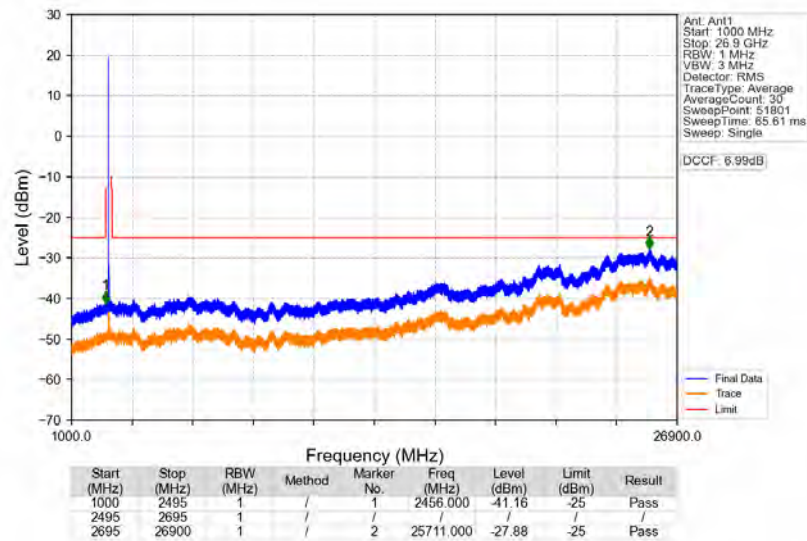
n41_30kHz_SISO_NTNV_40MHz_CP-OFDM_QPSK_2592.99MHz_Edge_1RB_Left
