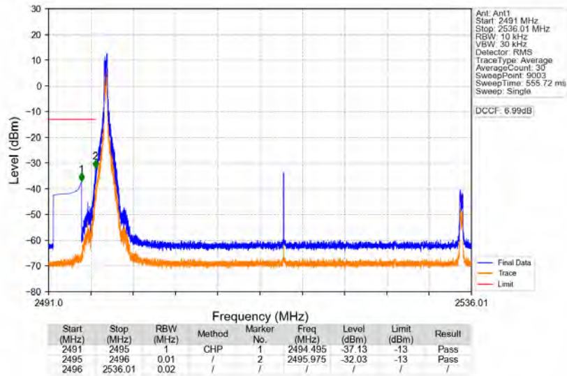
n41_30kHz_SISO_NTNV_40MHz_DFT-s-OFDM_QPSK_2516.01MHz_Edge_1RB_Left
