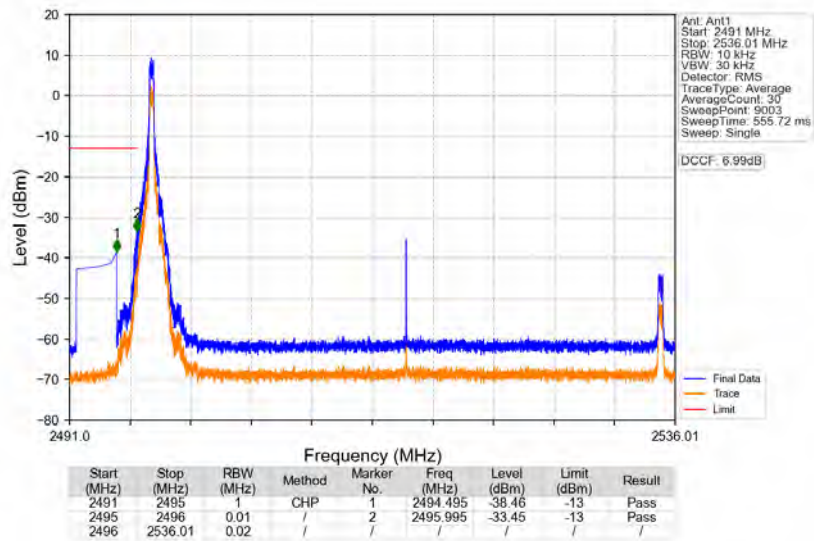
n41_30kHz_SISO_NTNV_40MHz_CP-OFDM_QPSK_2516.01MHz_Edge_1RB_Left
