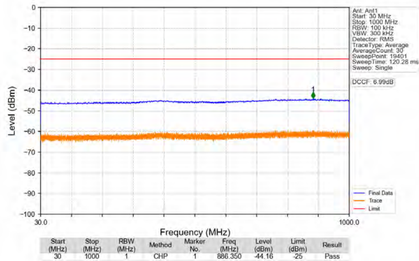
n41_30kHz_SISO_NTNV_60MHz_CP-OFDM_QPSK_2659.98MHz_Edge_1RB_Right
