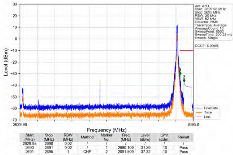
n41_30kHz_SISO_NTNV_60MHz_DFT-s-OFDM_QPSK_2659.98MHz_Edge_1RB_Right
