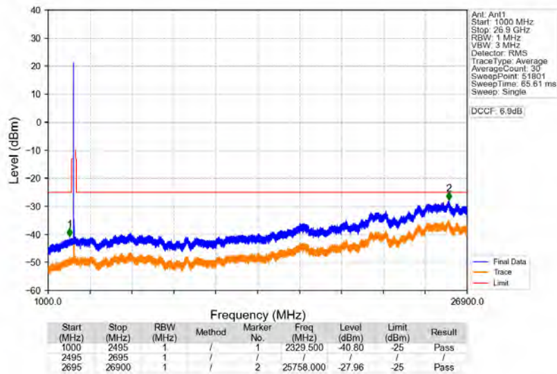
n41_30kHz_SISO_NTNV_50MHz_CP-OFDM_QPSK_2592.99MHz_Edge_1RB_Left
