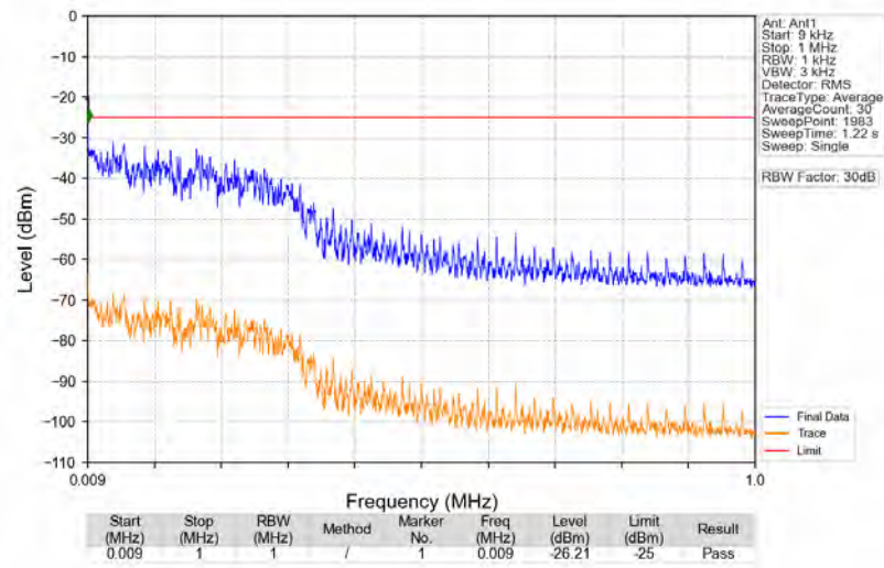
n41_30kHz_SISO_NTNV_40MHz_CP-OFDM_QPSK_2592.99MHz_Edge_1RB_Left
