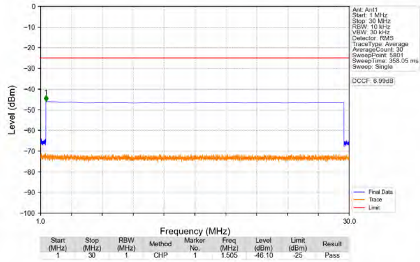
n41_30kHz_SISO_NTNV_40MHz_DFT-s-OFDM_PI/2_BPSK_2670MHz_Edge_1RB_Right
