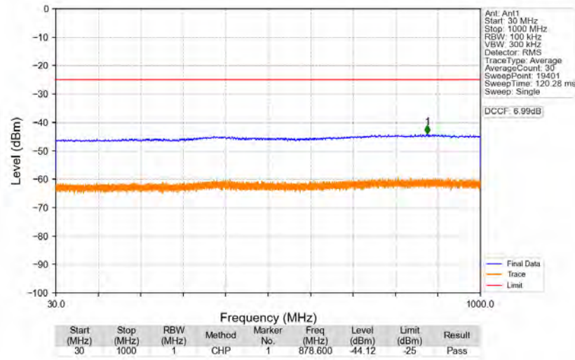
n41_30kHz_SISO_NTNV_70MHz_DFT-s-OFDM_QPSK_2592.99MHz_Edge_1RB_Left
