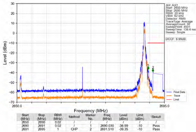
n41_30kHz_SISO_NTNV_40MHz_CP-OFDM_QPSK_2670MHz_Edge_1RB_Right
