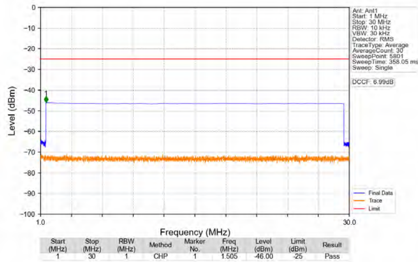
n41_30kHz_SISO_NTNV_40MHz_CP-OFDM_QPSK_2516.01MHz_Edge_1RB_Left
