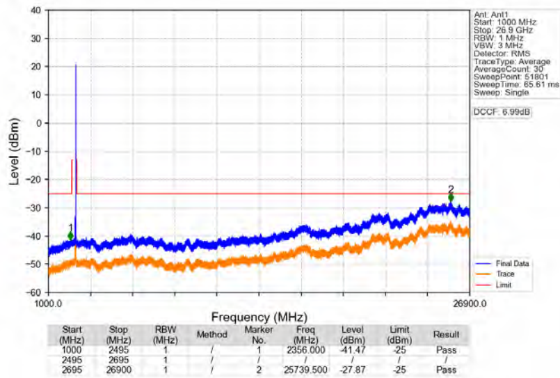
n41_30kHz_SISO_NTNV_60MHz_DFT-s-OFDM_QPSK_2659.98MHz_Edge_1RB_Right
