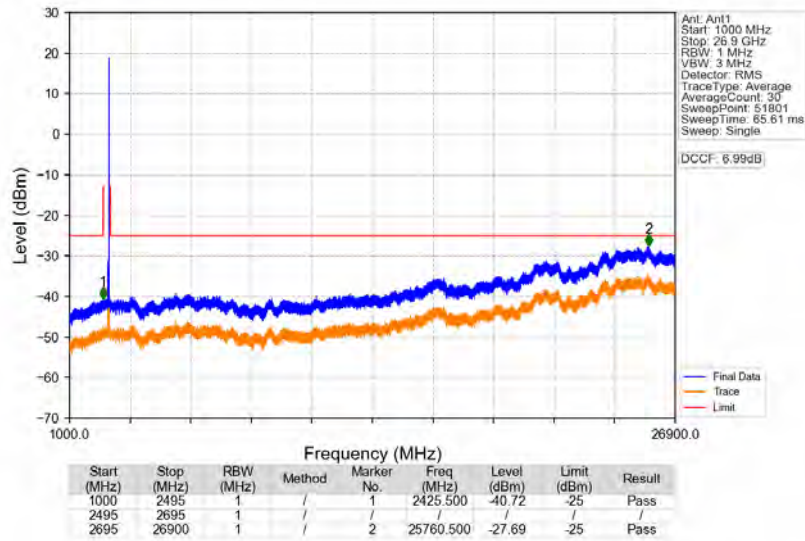
n41_30kHz_SISO_NTNV_60MHz_CP-OFDM_QPSK_2659.98MHz_Edge_1RB_Right
