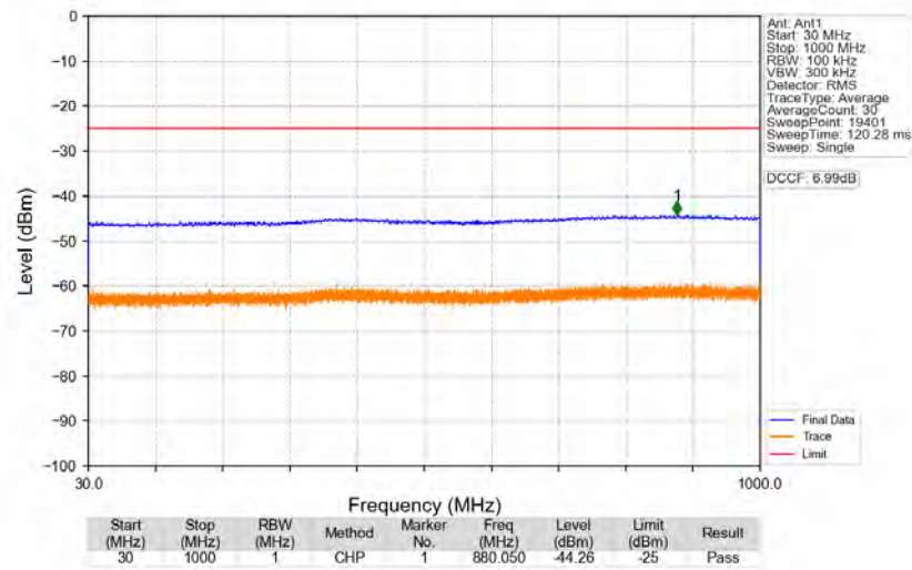
n41_30kHz_SISO_NTNV_70MHz_DFT-s-OFDM_QPSK_2531.01MHz_Edge_1RB_Left
