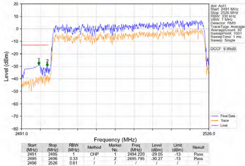
n41_30kHz_SISO_NTNV_30MHz_CP-OFDM_QPSK_2511MHz_Outer_Full
