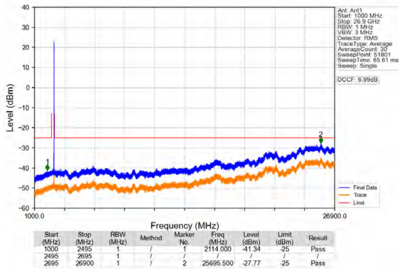
n41_30kHz_SISO_NTNV_30MHz_CP-OFDM_QPSK_2674.98MHz_Edge_1RB_Right
