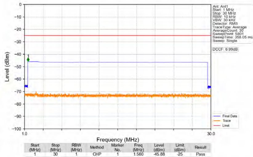
n41_30kHz_SISO_NTNV_60MHz_DFT-s-OFDM_QPSK_2592.99MHz_Edge_1RB_Left
