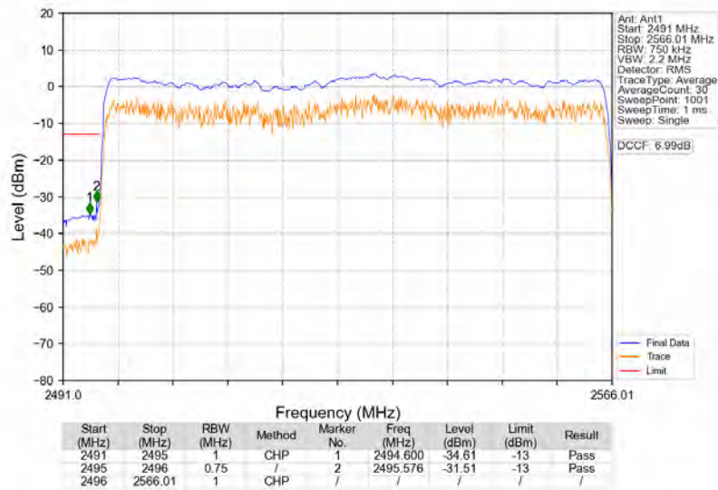
n41_30kHz_SISO_NTNV_70MHz_CP-OFDM_QPSK_2531.01MHz_Outer_Full
