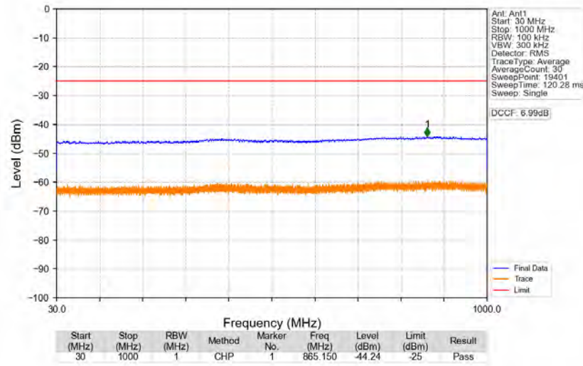
n41_30kHz_SISO_NTNV_30MHz_DFT-s-OFDM_QPSK_2592.99MHz_Edge_1RB_Left
