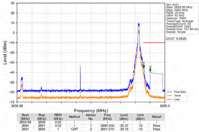
n41_30kHz_SISO_NTNV_30MHz_CP-OFDM_QPSK_2674.98MHz_Edge_1RB_Right
