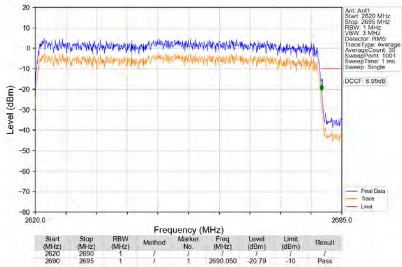
n41_30kHz_SISO_NTNV_70MHz_CP-OFDM_QPSK_2655MHz_Outer_Full
