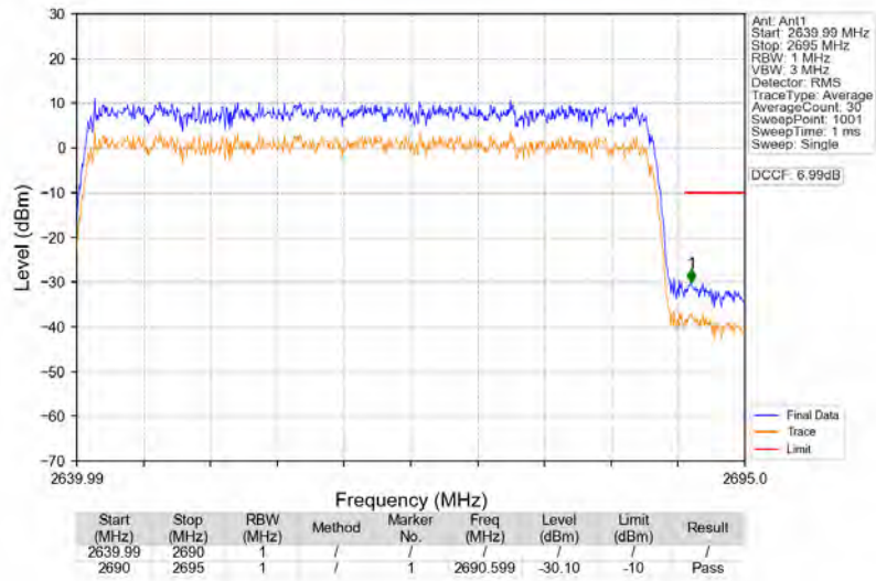
n41_30kHz_SISO_NTNV_50MHz_DFT-s-OFDM_PI/2_BPSK_2664.99MHz_Outer_Full
