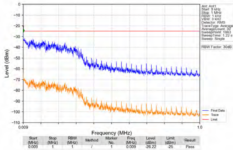
n41_30kHz_SISO_NTNV_30MHz_CP-OFDM_QPSK_2592.99MHz_Edge_1RB_Left
