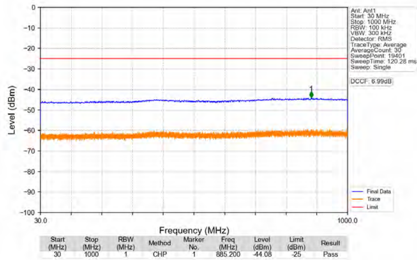
n41_30kHz_SISO_NTNV_40MHz_DFT-s-OFDM_QPSK_2516.01MHz_Edge_1RB_Left
