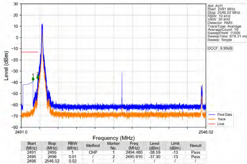
n41_30kHz_SISO_NTNV_50MHz_DFT-s-OFDM_QPSK_2521.02MHz_Edge_1RB_Left
