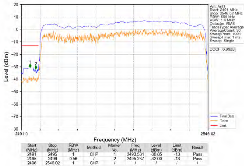
n41_30kHz_SISO_NTNV_50MHz_CP-OFDM_QPSK_2521.02MHz_Outer_Full
