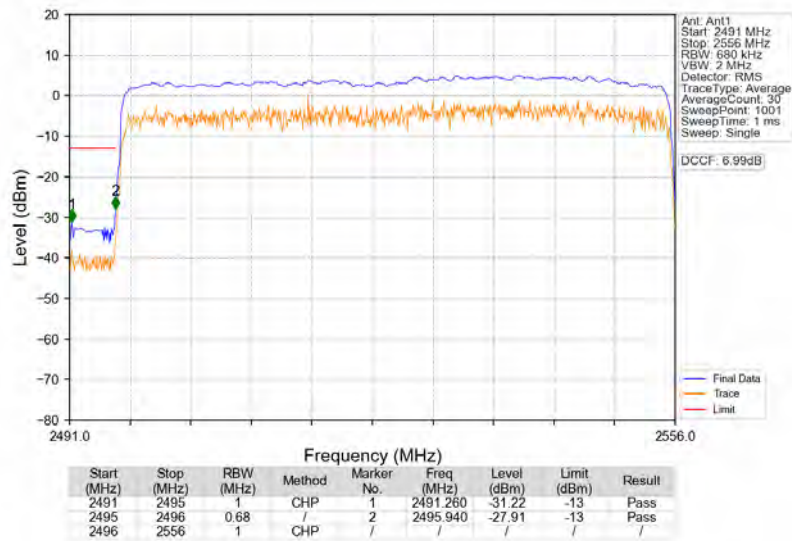
n41_30kHz_SISO_NTNV_60MHz_CP-OFDM_QPSK_2526MHz_Outer_Full
