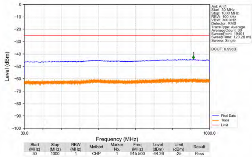
n41_30kHz_SISO_NTNV_40MHz_CP-OFDM_QPSK_2670MHz_Edge_1RB_Right
