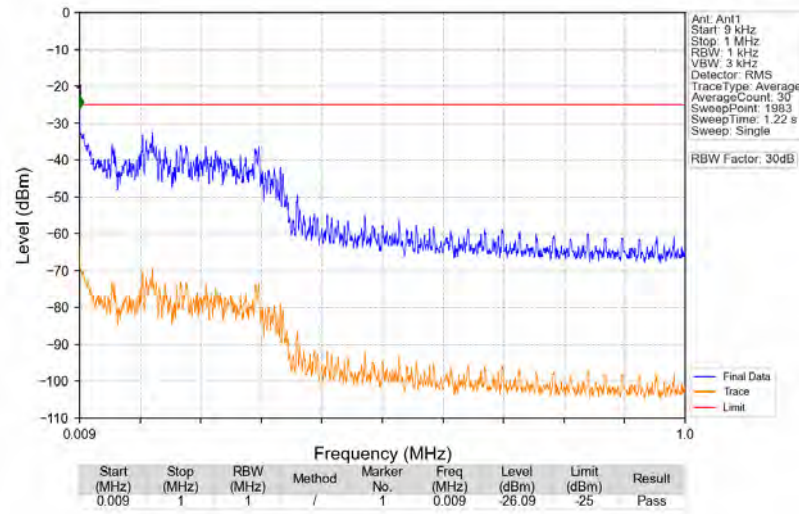
n41_30kHz_SISO_NTNV_30MHz_DFT-s-OFDM_QPSK_2592.99MHz_Edge_1RB_Left
