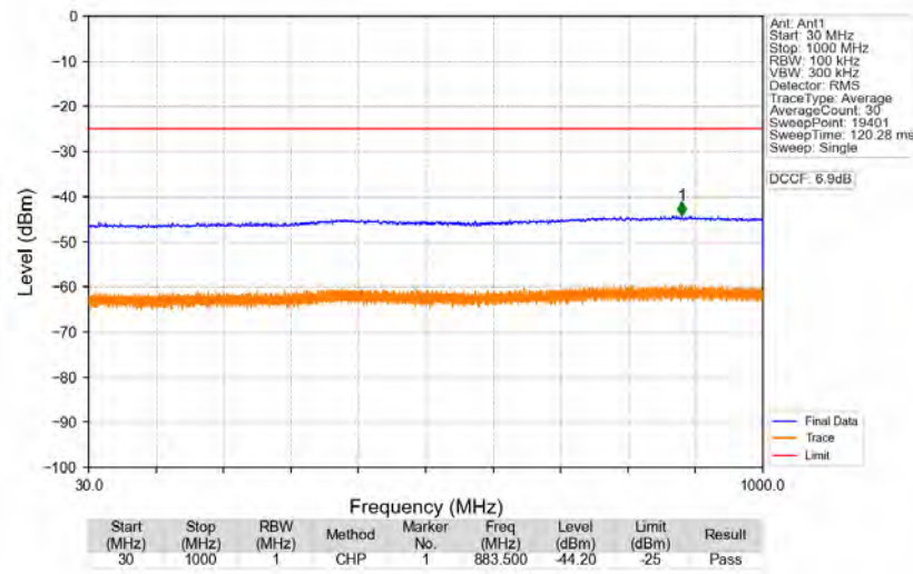
n41_30kHz_SISO_NTNV_50MHz_CP-OFDM_QPSK_2592.99MHz_Edge_1RB_Left
