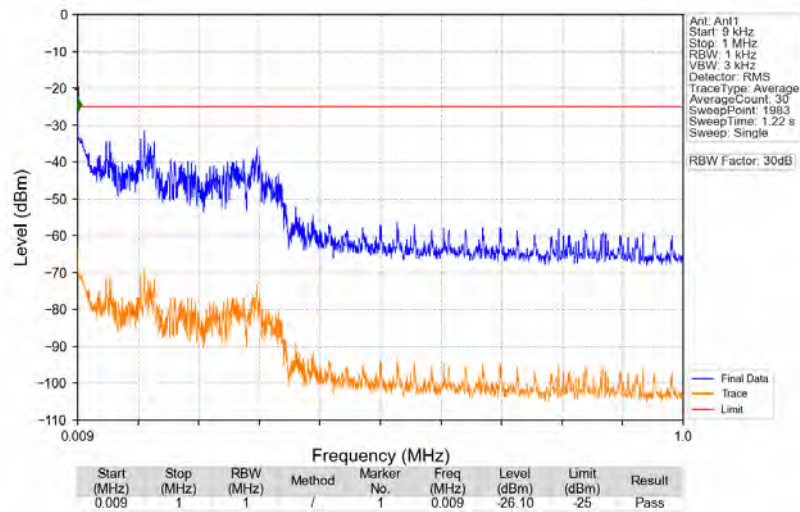
n41_30kHz_SISO_NTNV_40MHz_DFT-s-OFDM_PI/2_BPSK_2670MHz_Edge_1RB_Right
