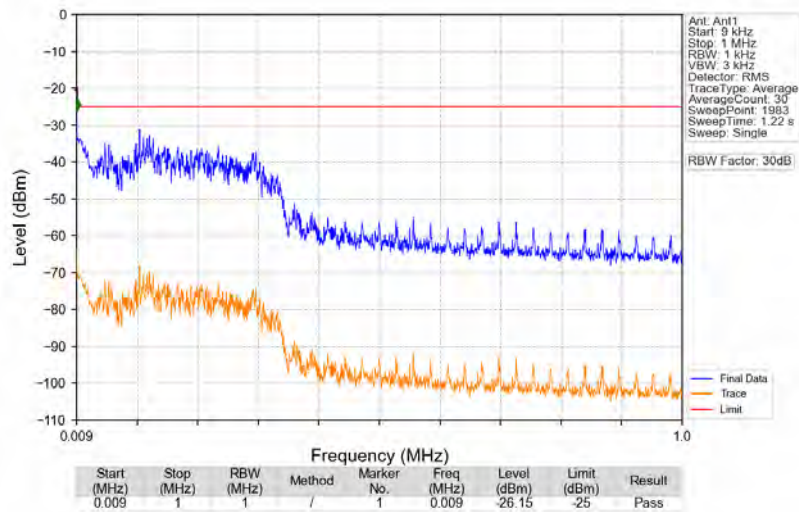
n41_30kHz_SISO_NTNV_60MHz_DFT-s-OFDM_QPSK_2659.98MHz_Edge_1RB_Right
