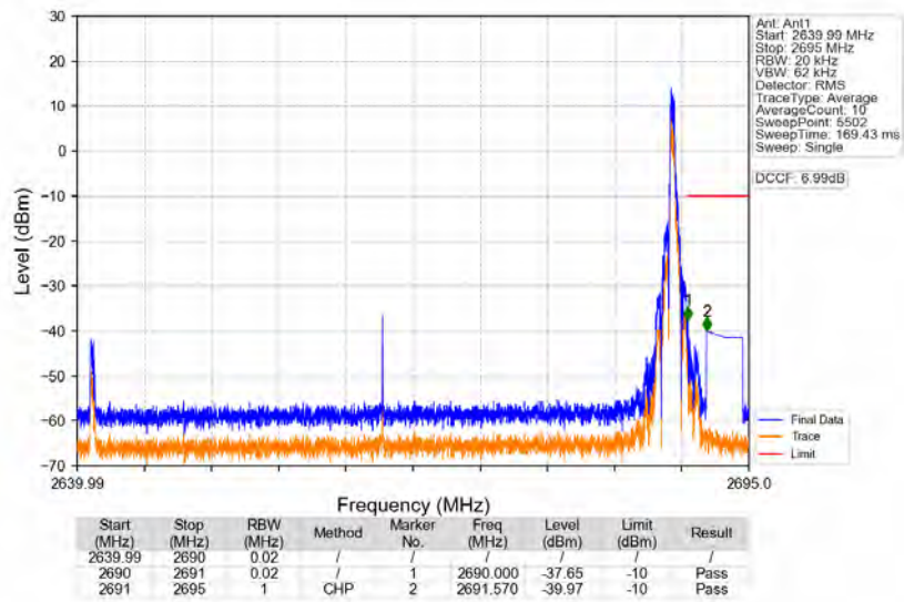
n41_30kHz_SISO_NTNV_50MHz_DFT-s-OFDM_QPSK_2664.99MHz_Edge_1RB_Right
