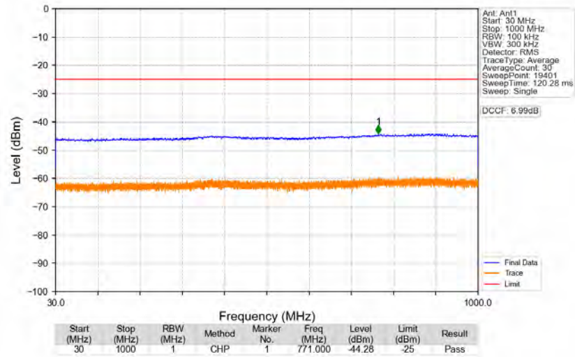
n41_30kHz_SISO_NTNV_30MHz_CP-OFDM_QPSK_2674.98MHz_Edge_1RB_Right
