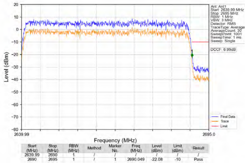
n41_30kHz_SISO_NTNV_50MHz_CP-OFDM_QPSK_2664.99MHz_Outer_Full
