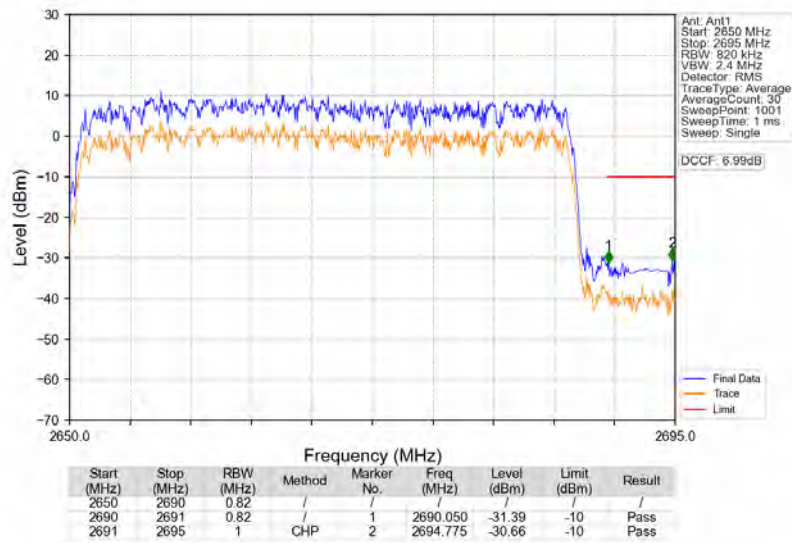
n41_30kHz_SISO_NTNV_40MHz_DFT-s-OFDM_QPSK_2670MHz_Outer_Full
