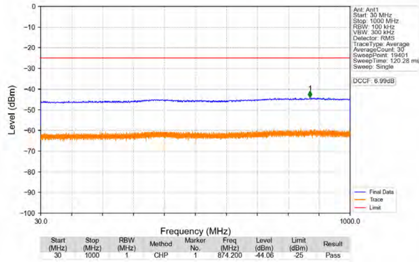
n41_30kHz_SISO_NTNV_30MHz_CP-OFDM_QPSK_2592.99MHz_Edge_1RB_Left
