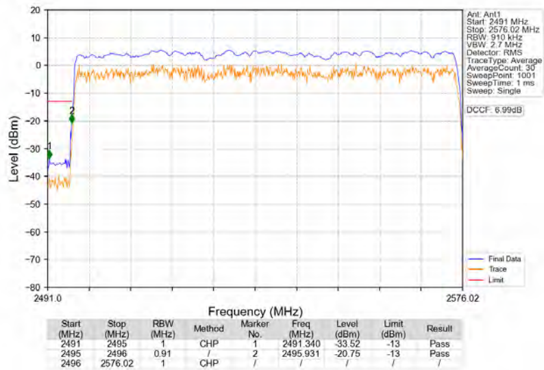
n41_30kHz_SISO_NTNV_80MHz_DFT-s-OFDM_PI/2_BPSK_2536.02MHz_Outer_Full
