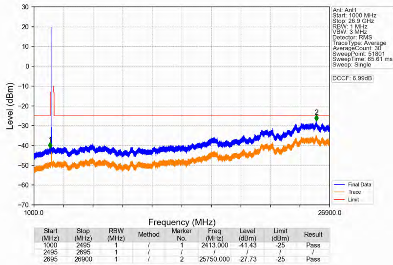
n41_30kHz_SISO_NTNV_70MHz_DFT-s-OFDM_QPSK_2531.01MHz_Edge_1RB_Left
