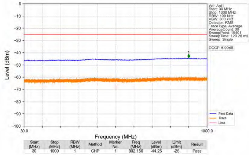
n41_30kHz_SISO_NTNV_70MHz_CP-OFDM_QPSK_2592.99MHz_Edge_1RB_Left
