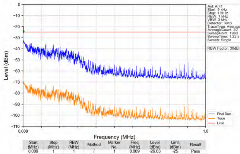
n41_30kHz_SISO_NTNV_30MHz_CP-OFDM_QPSK_2511MHz_Edge_1RB_Left
