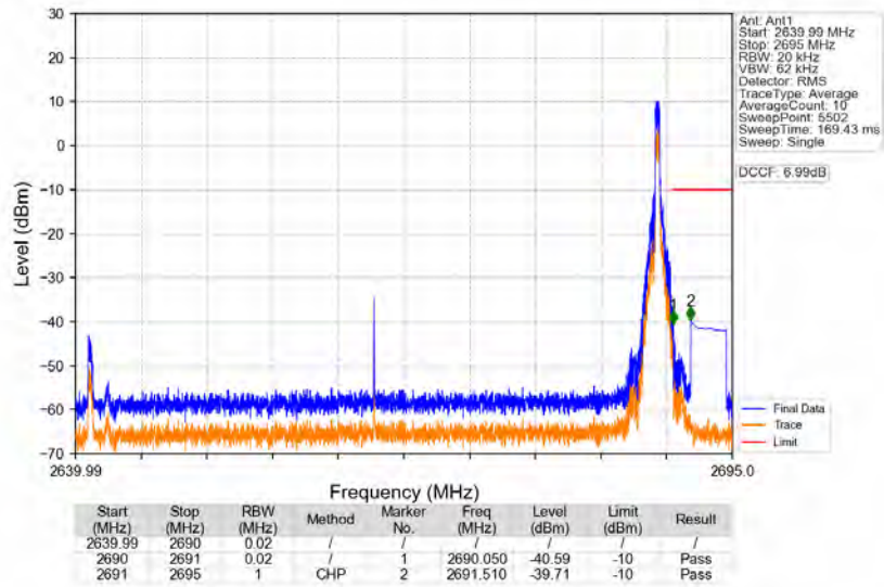
n41_30kHz_SISO_NTNV_50MHz_CP-OFDM_QPSK_2664.99MHz_Edge_1RB_Right
