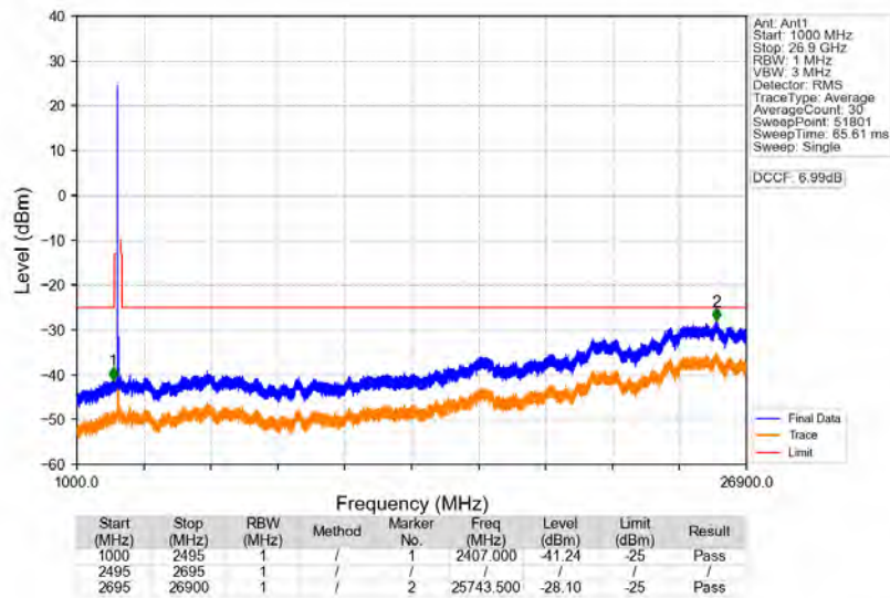
n41_30kHz_SISO_NTNV_50MHz_DFT-s-OFDM_QPSK_2592.99MHz_Edge_1RB_Left
