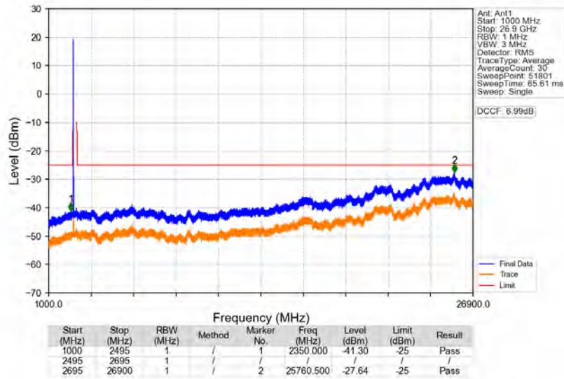
n41_30kHz_SISO_NTNV_40MHz_CP-OFDM_QPSK_2516.01MHz_Edge_1RB_Left
