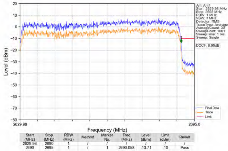
n41_30kHz_SISO_NTNV_60MHz_CP-OFDM_QPSK_2659.98MHz_Outer_Full
