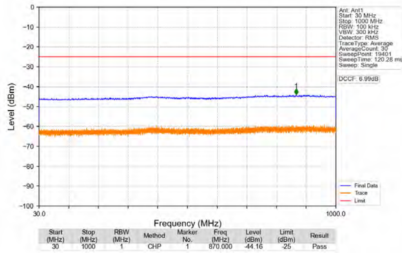
n41_30kHz_SISO_NTNV_50MHz_DFT-s-OFDM_QPSK_2592.99MHz_Edge_1RB_Left
