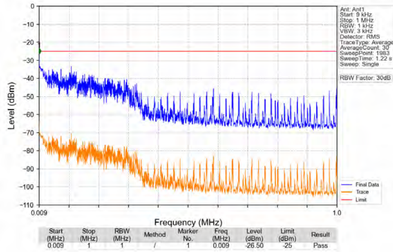
n41_30kHz_SISO_NTNV_70MHz_CP-OFDM_QPSK_2592.99MHz_Edge_1RB_Left
