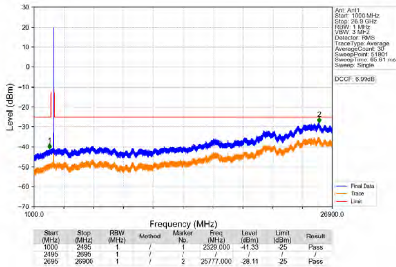
n41_30kHz_SISO_NTNV_50MHz_CP-OFDM_QPSK_2664.99MHz_Edge_1RB_Right
