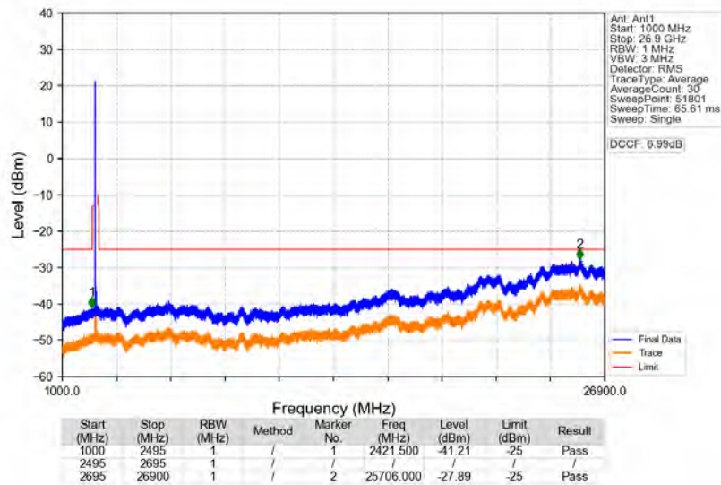
n41_30kHz_SISO_NTNV_60MHz_DFT-s-OFDM_QPSK_2592.99MHz_Edge_1RB_Left
