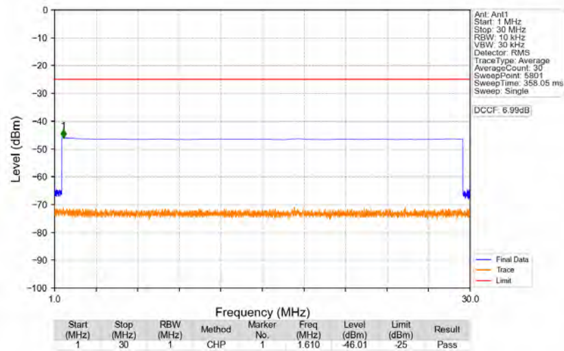
n41_30kHz_SISO_NTNV_30MHz_DFT-s-OFDM_QPSK_2592.99MHz_Edge_1RB_Left
