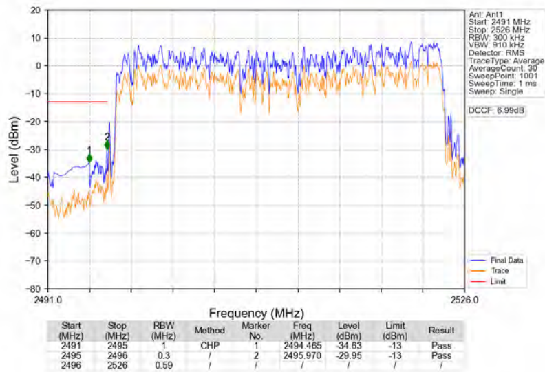
n41_30kHz_SISO_NTNV_30MHz_DFT-s-OFDM_QPSK_2511MHz_Outer_Full
