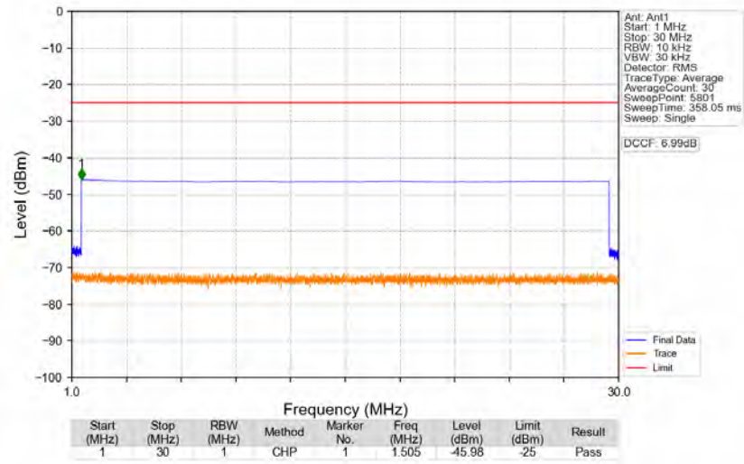
n41_30kHz_SISO_NTNV_30MHz_CP-OFDM_QPSK_2674.98MHz_Edge_1RB_Right
