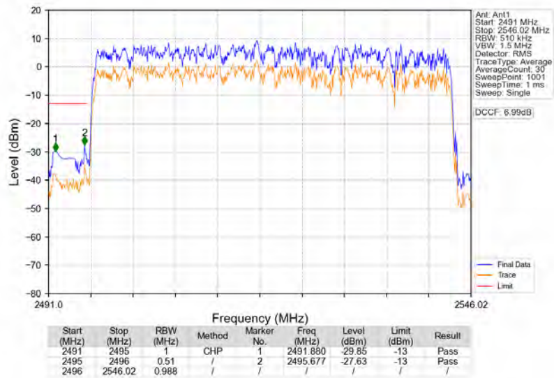
n41_30kHz_SISO_NTNV_50MHz_DFT-s-OFDM_PI/2_BPSK_2521.02MHz_Outer_Full
