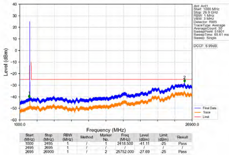
n41_30kHz_SISO_NTNV_40MHz_DFT-s-OFDM_PI/2_BPSK_2516.01MHz_Edge_1RB_Left
