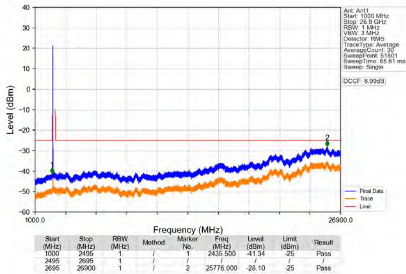
n41_30kHz_SISO_NTNV_40MHz_DFT-s-OFDM_QPSK_2516.01MHz_Edge_1RB_Left
