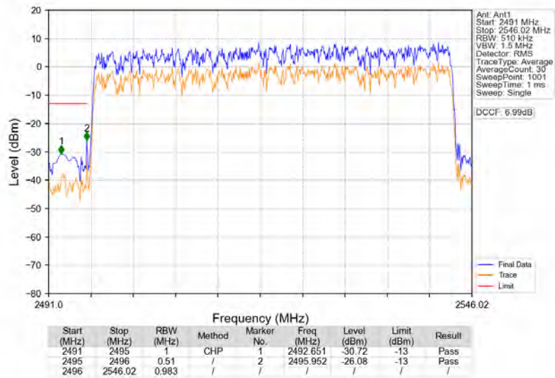
n41_30kHz_SISO_NTNV_50MHz_DFT-s-OFDM_QPSK_2521.02MHz_Outer_Full
