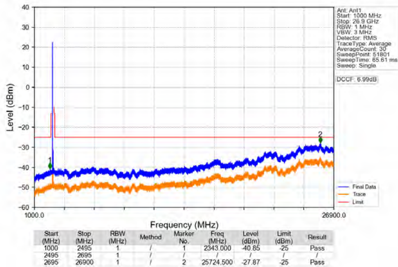
n41_30kHz_SISO_NTNV_70MHz_DFT-s-OFDM_QPSK_2592.99MHz_Edge_1RB_Left
