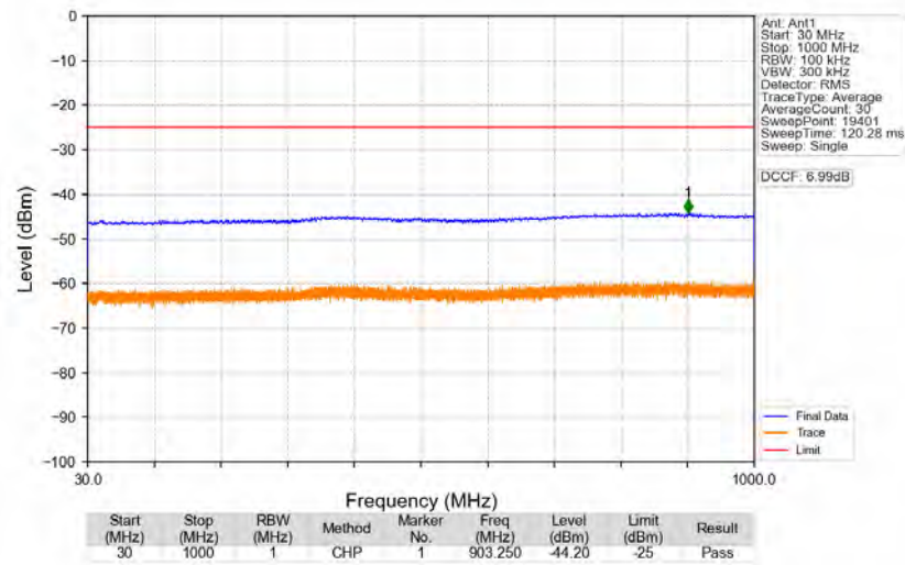
n41_30kHz_SISO_NTNV_80MHz_DFT-s-OFDM_QPSK_2536.02MHz_Edge_1RB_Left
