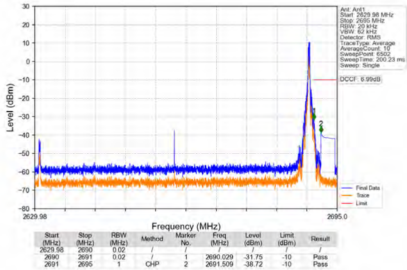
n41_30kHz_SISO_NTNV_60MHz_CP-OFDM_QPSK_2659.98MHz_Edge_1RB_Right
