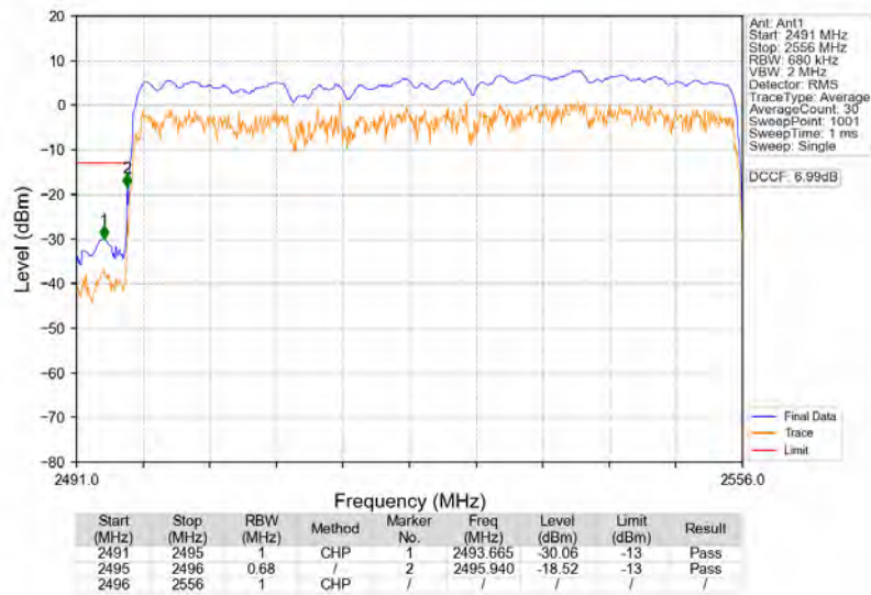
n41_30kHz_SISO_NTNV_60MHz_DFT-s-OFDM_QPSK_2526MHz_Outer_Full
