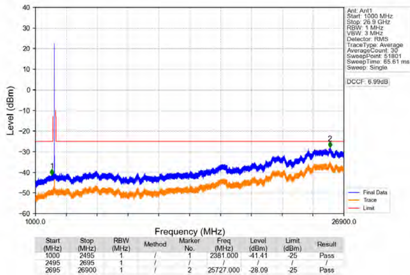
n41_30kHz_SISO_NTNV_30MHz_DFT-s-OFDM_QPSK_2592.99MHz_Edge_1RB_Left
