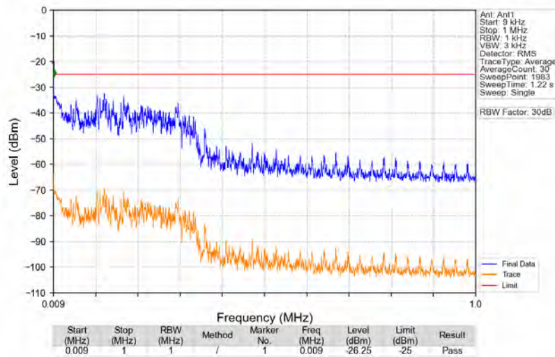
n41_30kHz_SISO_NTNV_80MHz_DFT-s-OFDM_QPSK_2536.02MHz_Edge_1RB_Left
