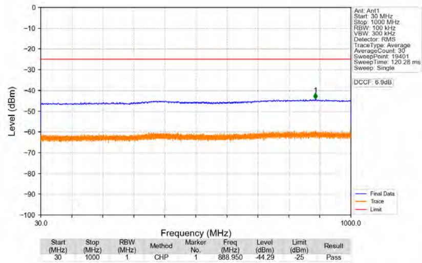
n41_30kHz_SISO_NTNV_40MHz_DFT-s-OFDM_QPSK_2670MHz_Edge_1RB_Right
