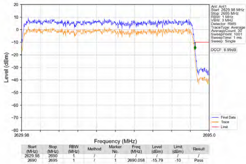
n41_30kHz_SISO_NTNV_60MHz_DFT-s-OFDM_PI/2_BPSK_2659.98MHz_Outer_Full
