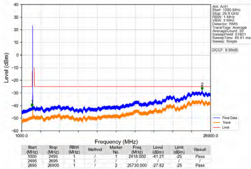
n41_30kHz_SISO_NTNV_50MHz_DFT-s-OFDM_QPSK_2521.02MHz_Edge_1RB_Left
