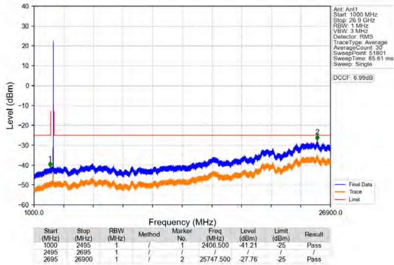
n41_30kHz_SISO_NTNV_50MHz_DFT-s-OFDM_PI/2_BPSK_2664.99MHz_Edge_1RB_Right
