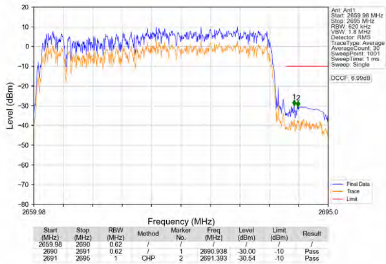
n41_30kHz_SISO_NTNV_30MHz_DFT-s-OFDM_QPSK_2674.98MHz_Outer_Full
