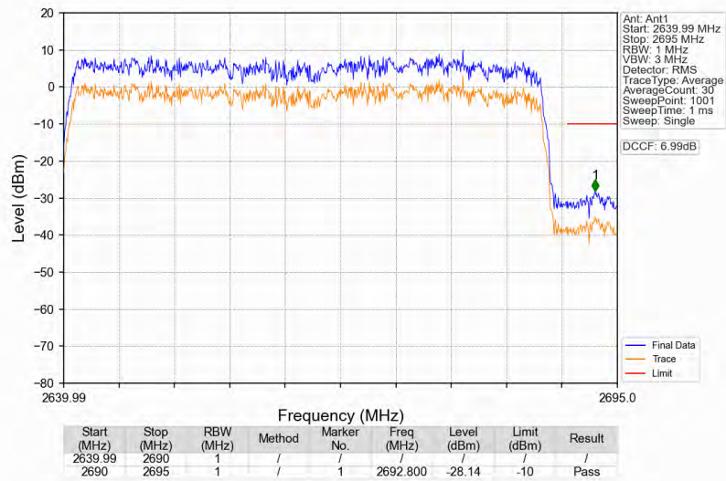
n41_30kHz_SISO_NTNV_50MHz_DFT-s-OFDM_QPSK_2664.99MHz_Outer_Full
