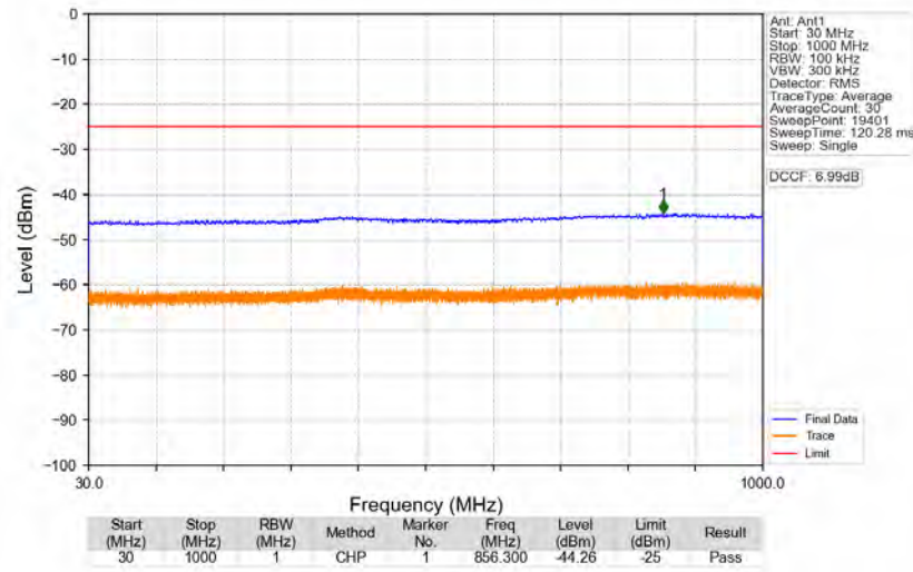
n41_30kHz_SISO_NTNV_60MHz_DFT-s-OFDM_QPSK_2592.99MHz_Edge_1RB_Left
