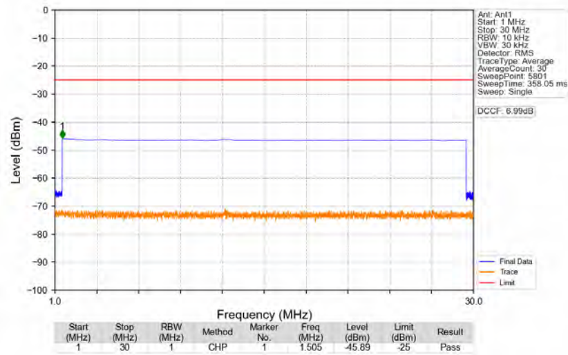
n41_30kHz_SISO_NTNV_40MHz_DFT-s-OFDM_QPSK_2592.99MHz_Edge_1RB_Left
