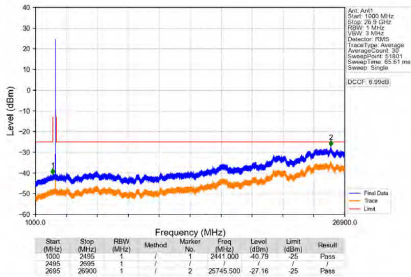
n41_30kHz_SISO_NTNV_50MHz_DFT-s-OFDM_QPSK_2664.99MHz_Edge_1RB_Right
