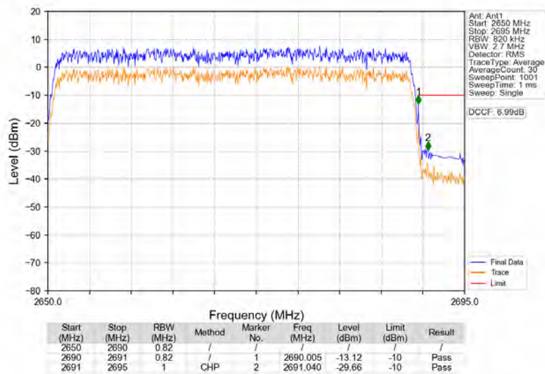
n41_30kHz_SISO_NTNV_40MHz_CP-OFDM_QPSK_2670MHz_Outer_Full
