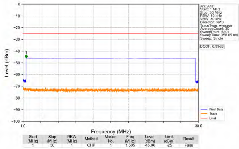
n41_30kHz_SISO_NTNV_50MHz_CP-OFDM_QPSK_2664.99MHz_Edge_1RB_Right
