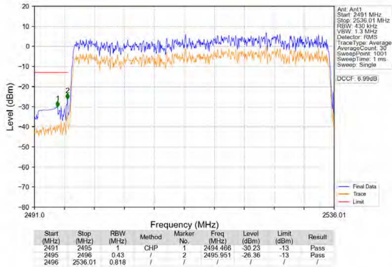
n41_30kHz_SISO_NTNV_40MHz_CP-OFDM_QPSK_2516.01MHz_Outer_Full
