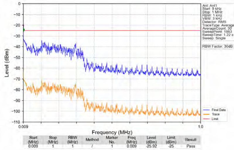
n41_30kHz_SISO_NTNV_60MHz_DFT-s-OFDM_QPSK_2592.99MHz_Edge_1RB_Left
