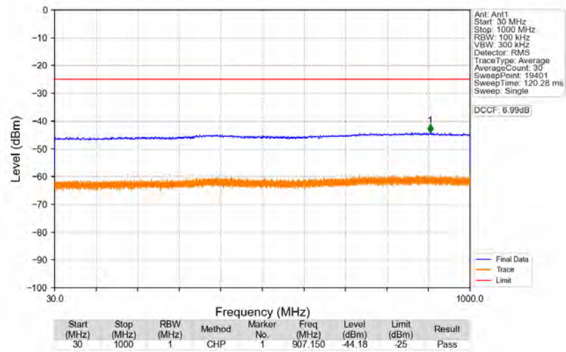
n41_30kHz_SISO_NTNV_30MHz_CP-OFDM_QPSK_2511MHz_Edge_1RB_Left
