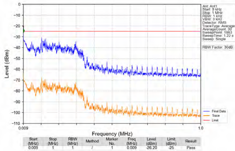
n41_30kHz_SISO_NTNV_70MHz_DFT-s-OFDM_QPSK_2592.99MHz_Edge_1RB_Left
