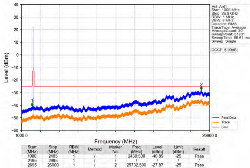
n41_30kHz_SISO_NTNV_30MHz_CP-OFDM_QPSK_2592.99MHz_Edge_1RB_Left
