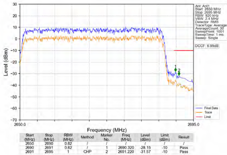
n41_30kHz_SISO_NTNV_40MHz_DFT-s-OFDM_PI/2_BPSK_2670MHz_Outer_Full
