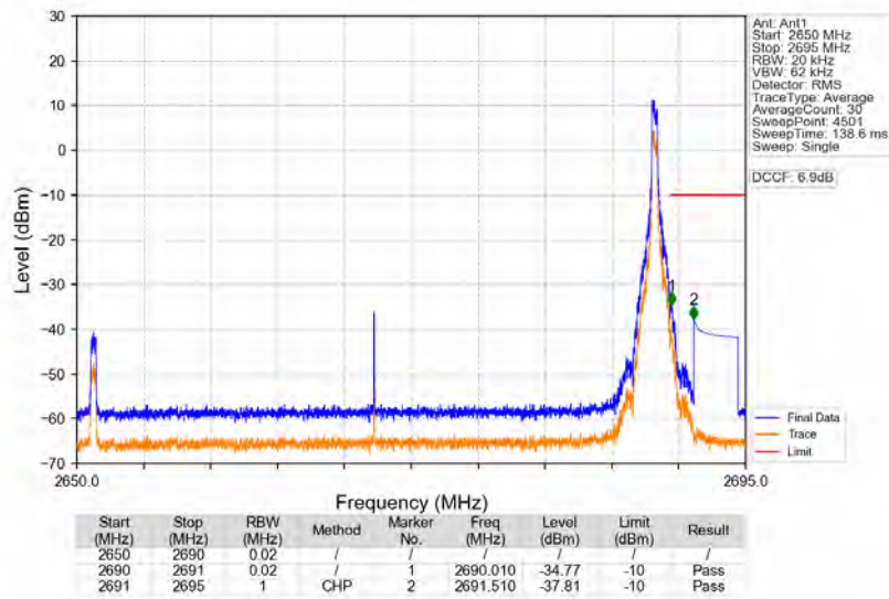
n41_30kHz_SISO_NTNV_40MHz_DFT-s-OFDM_QPSK_2670MHz_Edge_1RB_Right
