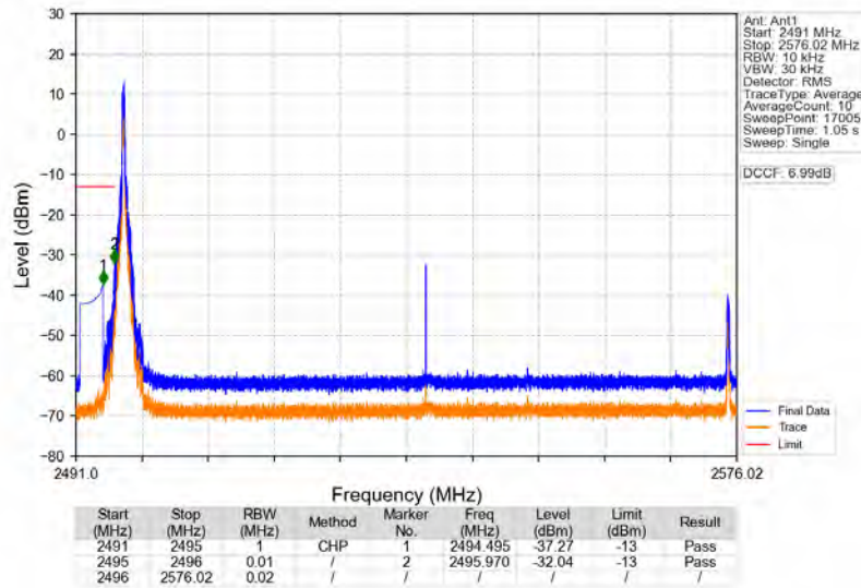
n41_30kHz_SISO_NTNV_80MHz_DFT-s-OFDM_QPSK_2536.02MHz_Edge_1RB_Left
