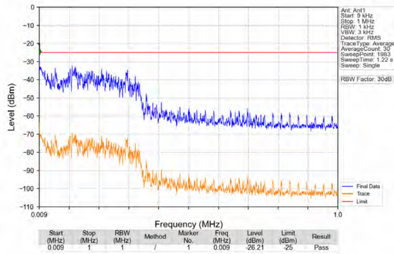
n41_30kHz_SISO_NTNV_40MHz_DFT-s-OFDM_QPSK_2592.99MHz_Edge_1RB_Left
