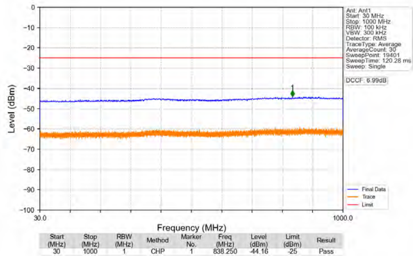
n41_30kHz_SISO_NTNV_50MHz_DFT-s-OFDM_QPSK_2521.02MHz_Edge_1RB_Left
