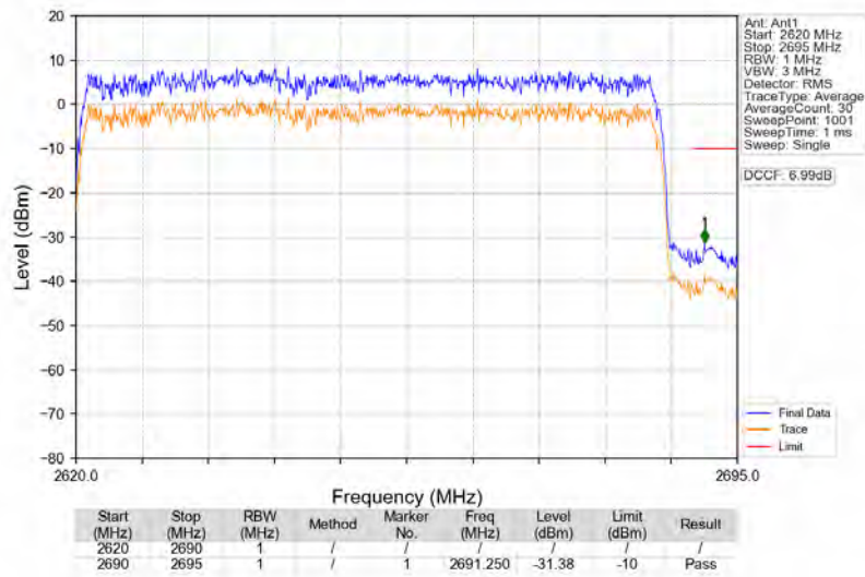
n41_30kHz_SISO_NTNV_70MHz_DFT-s-OFDM_QPSK_2655MHz_Outer_Full
