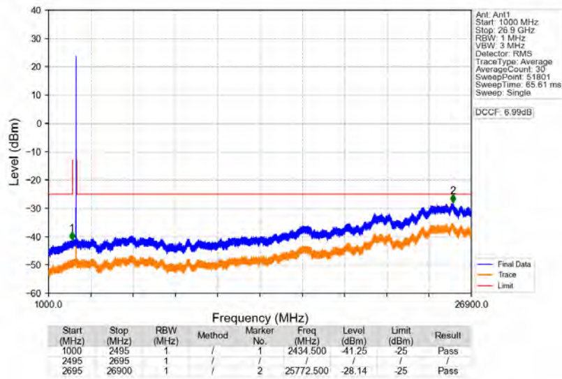
n41_30kHz_SISO_NTNV_30MHz_DFT-s-OFDM_QPSK_2674.98MHz_Edge_1RB_Right
