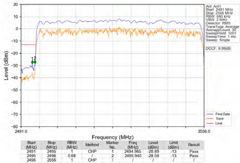
n41_30kHz_SISO_NTNV_60MHz_DFT-s-OFDM_PI/2_BPSK_2526MHz_Outer_Full
