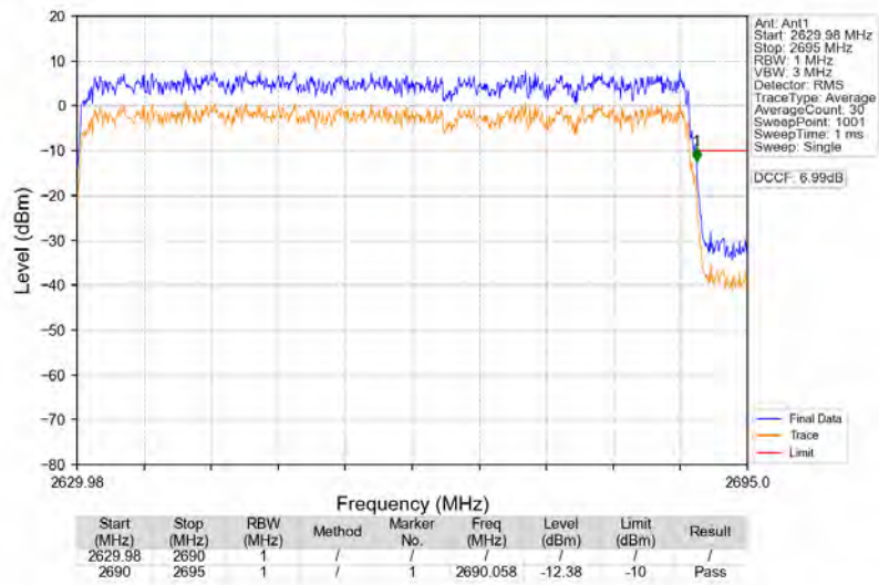
n41_30kHz_SISO_NTNV_60MHz_DFT-s-OFDM_QPSK_2659.98MHz_Outer_Full
