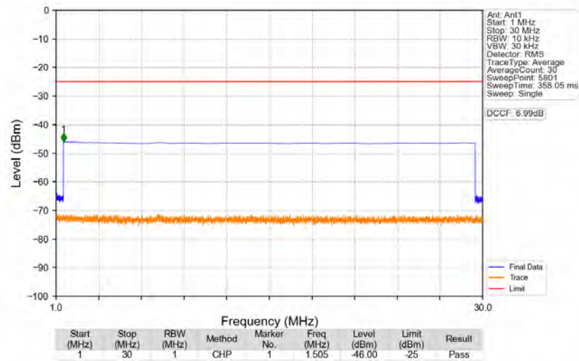
n41_30kHz_SISO_NTNV_50MHz_DFT-s-OFDM_QPSK_2592.99MHz_Edge_1RB_Left
