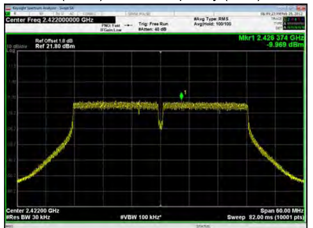
802.11n(HT40), Carrier frequency (MHz): 2422
