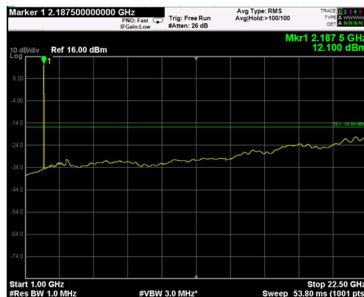
Channel: BOTTOM, Modulation: QPSK, BW=15MHz, Range: Upper
