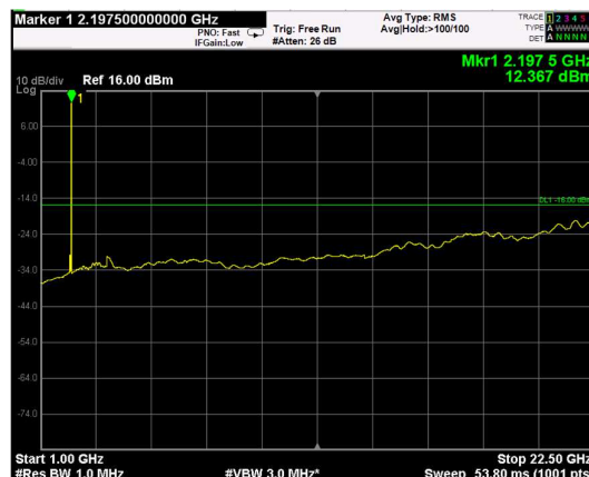
Channel: TOP, Modulation: 64QAM, BW=5MHz, Range: Upper
