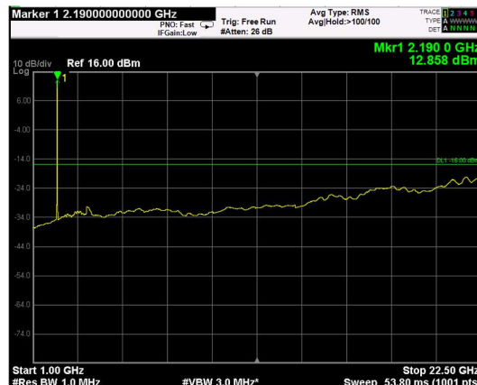
Channel: MIDDLE, Modulation: 64QAM, BW=5MHz, Range: Upper
