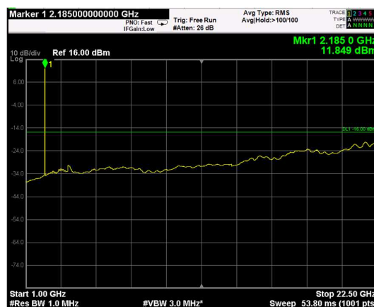
Channel: BOTTOM, Modulation: QPSK, BW=10MHz, Range: Upper
