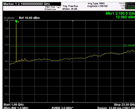
Channel: MIDDLE, Modulation: 16QAM, BW=10MHz, Range: Upper
