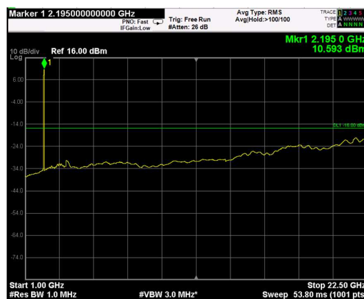
Channel: TOP, Modulation: QPSK, BW=10MHz, Range: Upper
