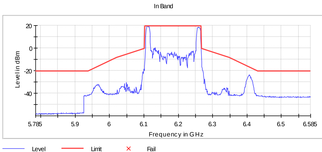
Figure 11: 6185 160MHz RU Vérification - Edge
