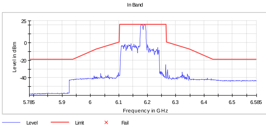
Figure 10: 6185 160MHz RU Vérification - Center
