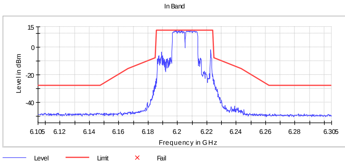
Figure 6: 6205 40MHz RU Vérification - Center
