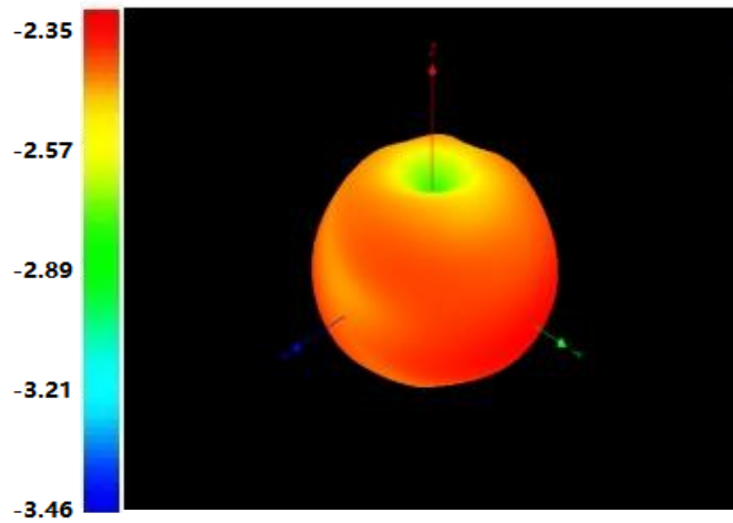
WIFI Antenna 3D Radiation Pattern
