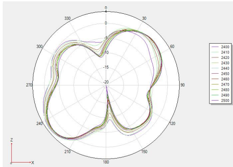
Phi 0 2D:
