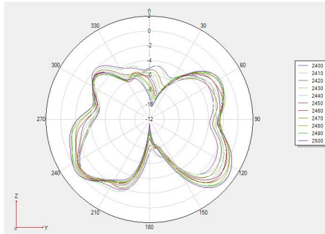
Phi 90 2D
