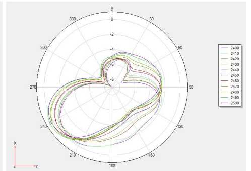
Theta 90 2D
