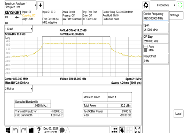
Band26-Part90s_1.4MHz_16QAM_RB6_0_CH26783
