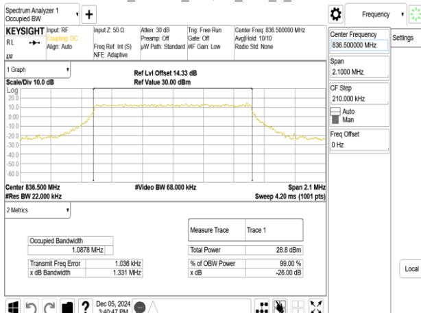
Band26_1.4MHz_64QAM_RB6_0_CH26915
