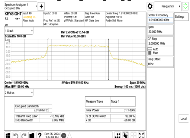
Band25_10MHz_16QAM_RB50_0_CH26640
