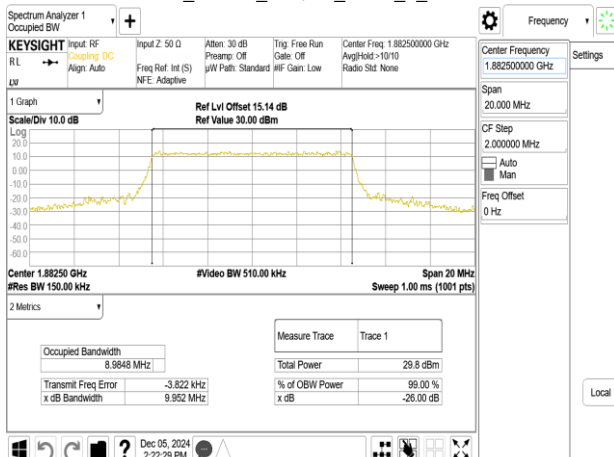
Band25_10MHz_64QAM_RB50_0_CH26365
