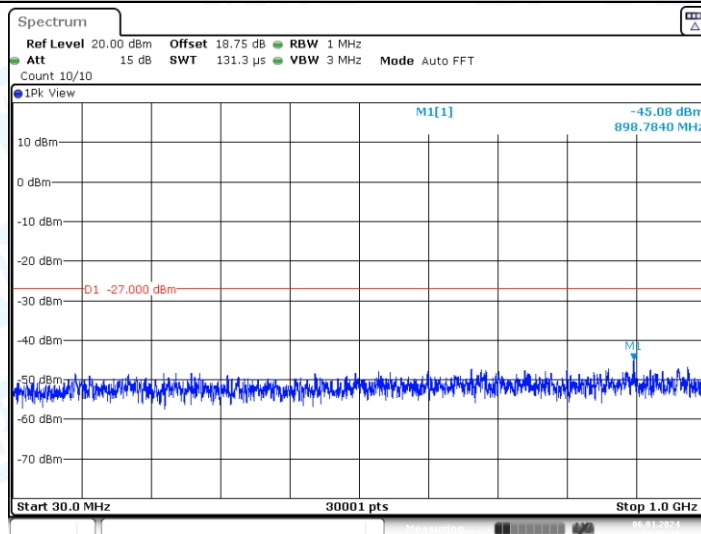
11AC20-CDD_Ant2_5745_30~1000
