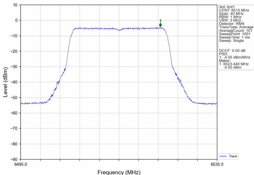
802.11ax(HEW20)_HCH_6515MHz_RU242_Left_Ant1_NTNV
