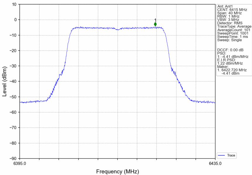
802.11ax(HEW20)_HCH_6415MHz_RU242_Left_Ant1_NTNV
