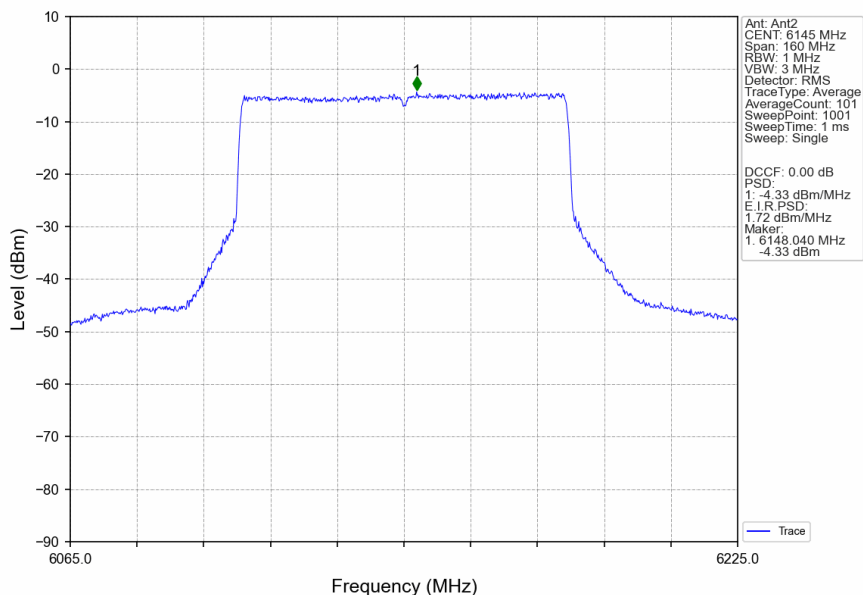
802.11ax(HEW80)_MCH_6145MHz_RU996_Left_Ant2_NTNV
