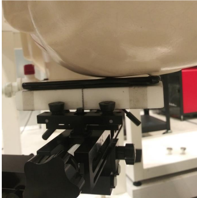
SAR Test Setup Photo 3: Left Cheek
