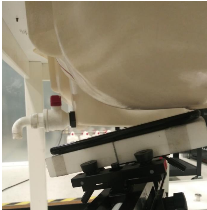
SAR Test Setup Photo 4: Left Tilt
