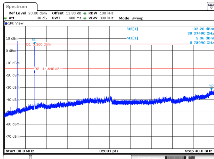
Conducted Emission Plot of Antenna port 1
