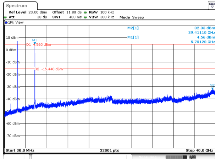
Conducted Emission Plot of Antenna port 0
