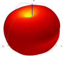
2490.0MHz H+V, ER: 78.6%
