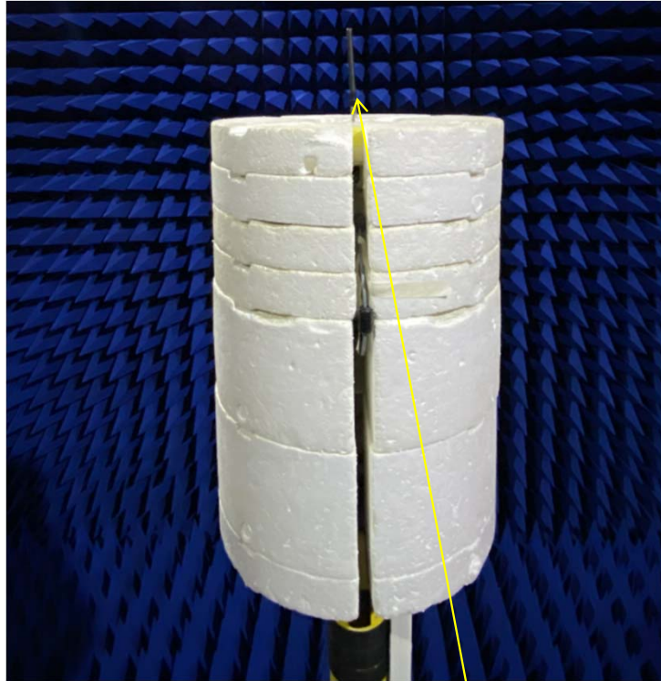
Testing environment
