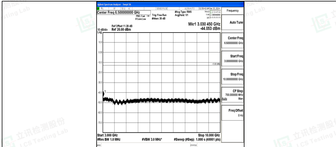
Band26_5MHz_QPSK_27015_1RB#0_3000~10000_3000~10000
