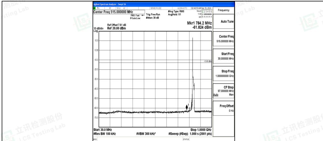
Band26_15MHz_16QAM_26965_1RB#0_30~1000_30~1000
