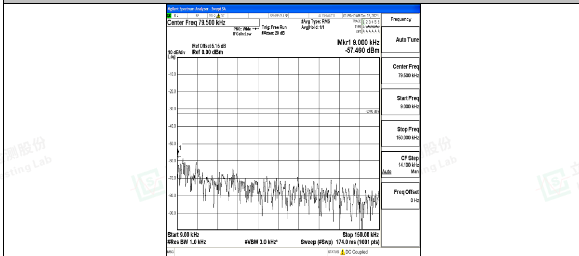
Band26_5MHz_16QAM_27015_1RB#0_0.009~0.15_0.009~0.15
