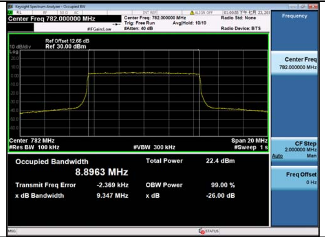
LTE band 13 - Low CH 16QAM-10
