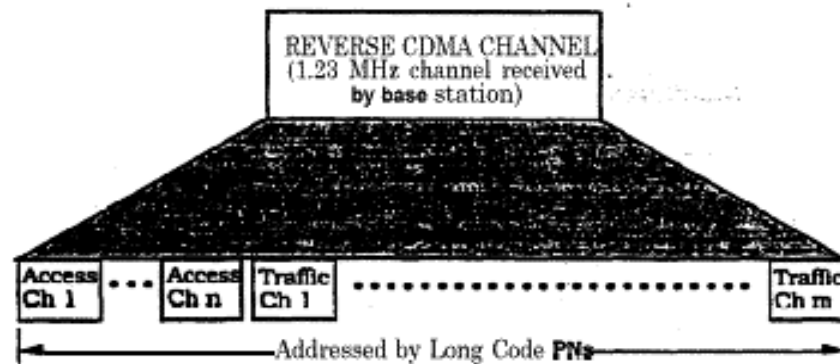
Figure 6.1.3.1-1. Example of Logical Reverse CDMA Channels Received at a Base Station
