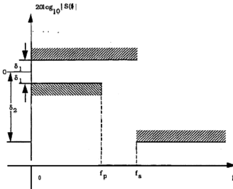
Figure 6.1.3.1.10-L Baseband Filters Frequency Response Limits
