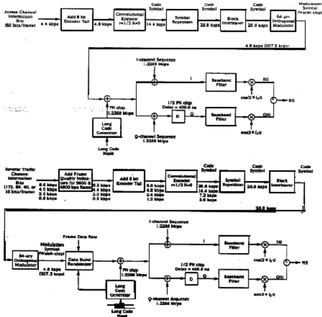
Figure 6.1.3.1-2. Reverse CDMA Channel Structure
