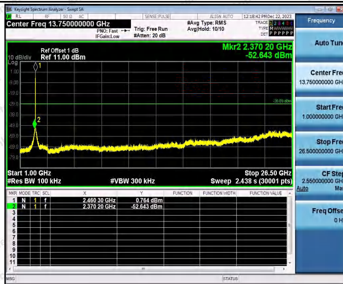
802.11g_Ant2_2462_0~Reference
