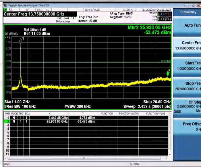
802.11n(HT40)SISO_Ant2_2437_0~Reference
