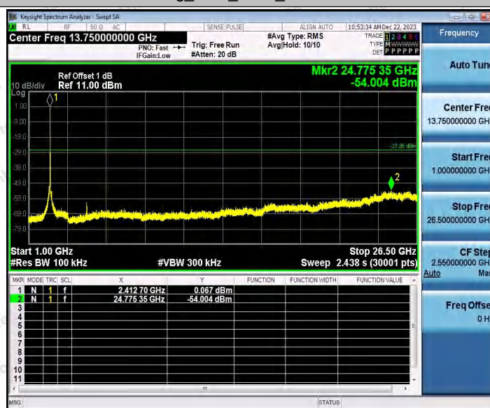
802.11g_Ant2_2412_0~Reference
