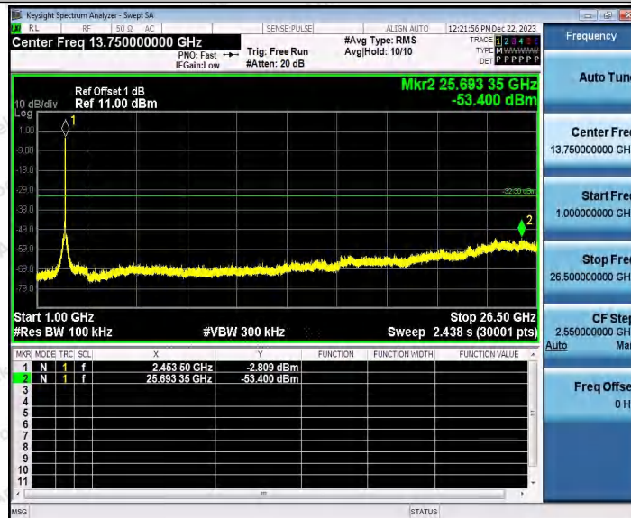
802.11n(HT40)SISO_Ant2_2452_0~Reference
