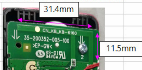
EL52219 HS Antenna Dimensions in mm
