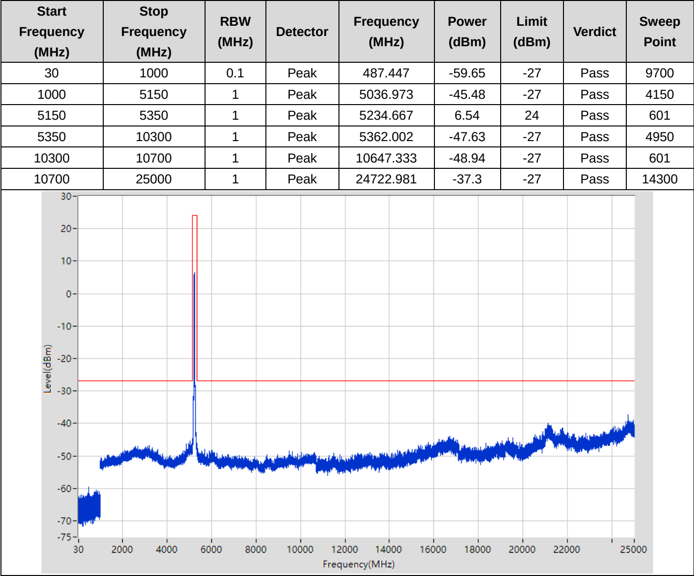
Chain 2 Undesirable Emission, 30MHz-25GHz, 802.11n(HT40), 5230MHz
