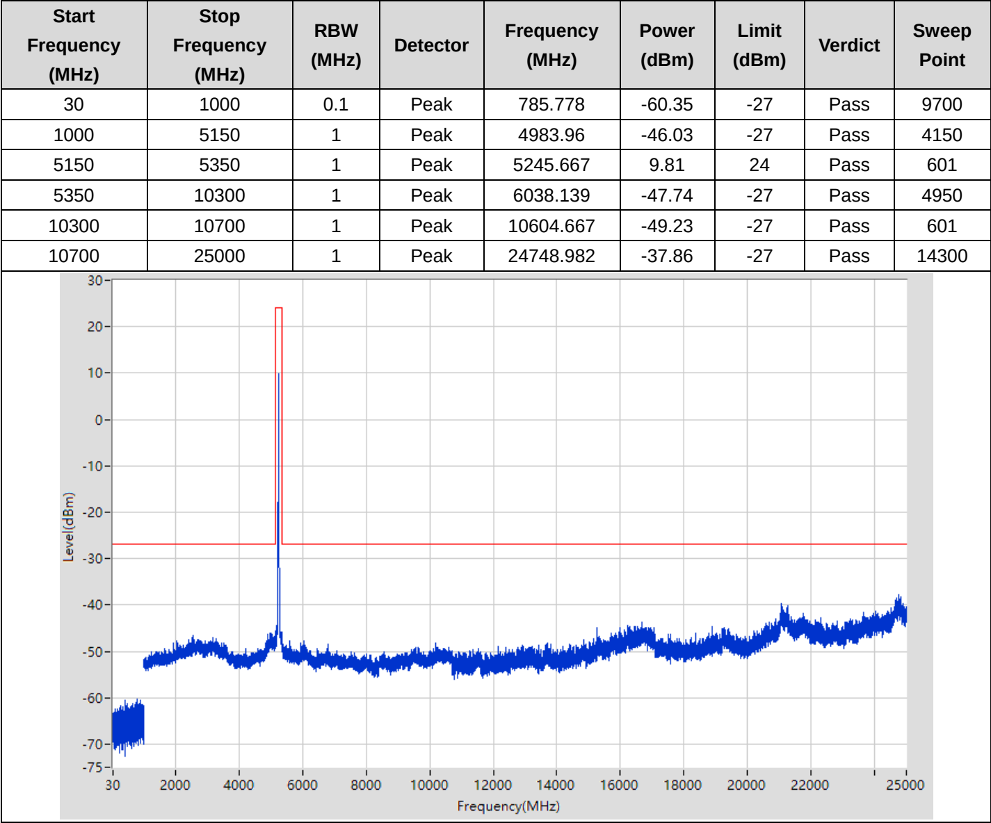
Chain 2 Undesirable Emission, 30MHz-25GHz, 802.11a, 5240MHz
