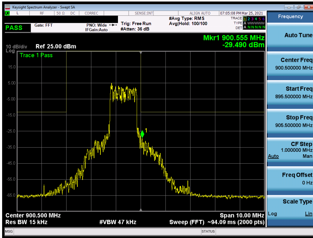
Plot 7-13. Upper Band Edge Plot (1.4MHz, QPSK, 6RB, RB Offset 0, NB=0)
