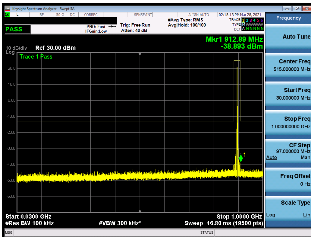
Plot 7-14. Conducted Spurious Plot – Low Channel (1.4MHz, QPSK, 1RB, RB Offset 0)
