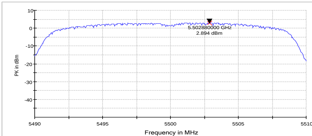
Channel 100 / 5500MHz (RBW: 1 MHz, VBW: 3 MHz)
