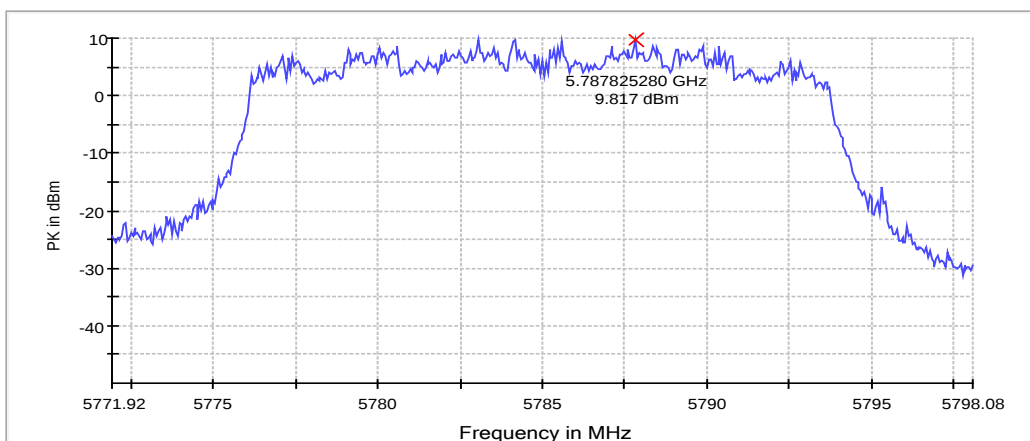
Channel 157 / 5785MHz (RBW: 500 kHz, VBW: 3 MHz)
