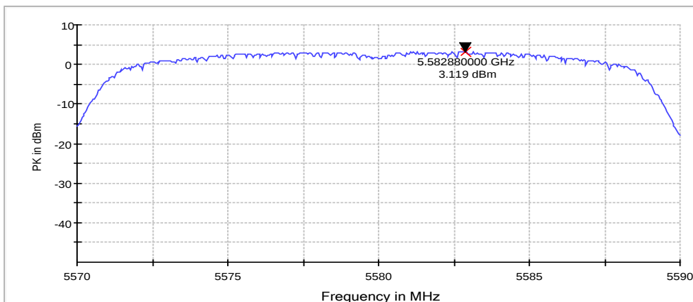
Channel 116 / 5580MHz (RBW: 1 MHz, VBW: 3 MHz)
