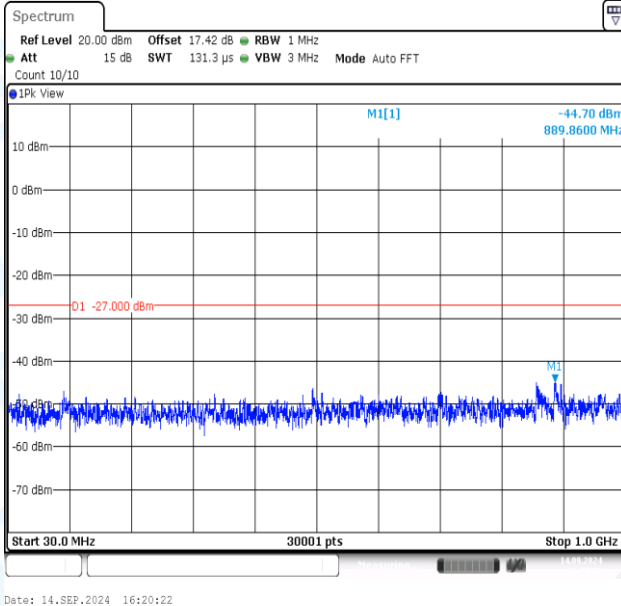
11N20MIMO-Ant1-5280-30~1000-PASS
