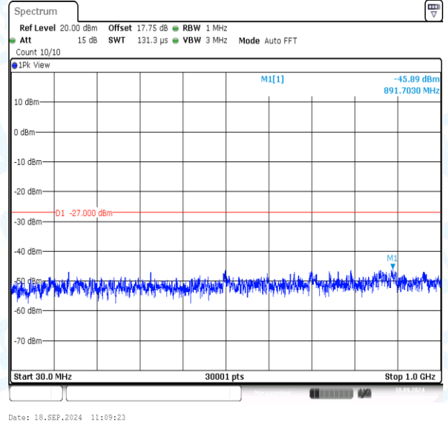
11N40MIMO-Ant2-5755-30~1000-PASS
