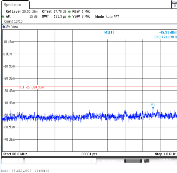
11N40MIMO-Ant1-5755-30~1000-PASS
