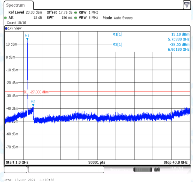
11N40MIMO-Ant2-5755-1000~40000-PASS
