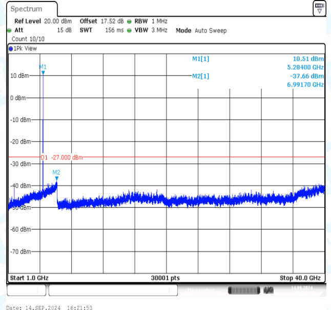
11N20MIMO-Ant2-5280-1000~40000-PASS
