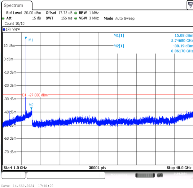
11N20MIMO-Ant1-5745-1000~40000-PASS
