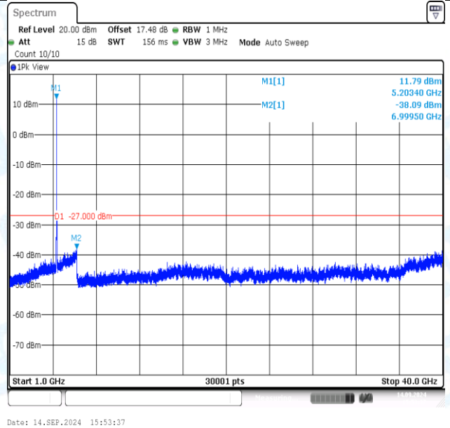
11N20MIMO-Ant2-5200-1000~40000-PASS
