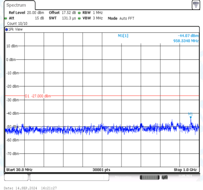
11N20MIMO-Ant2-5280-30~1000-PASS
