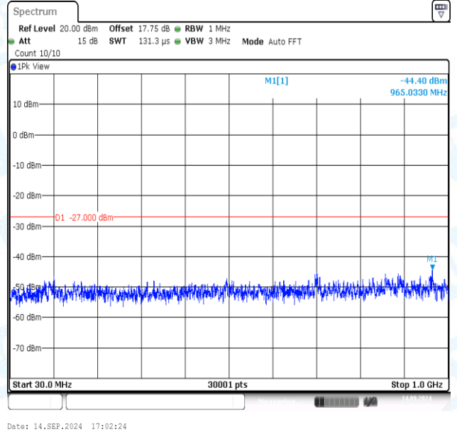
11N20MIMO-Ant2-5745-30~1000-PASS
