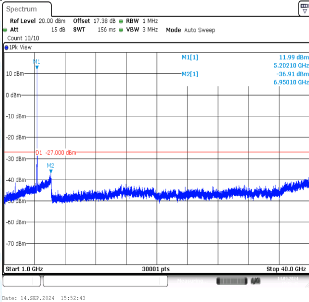
11N20MIMO-Ant1-5200-1000~40000-PASS
