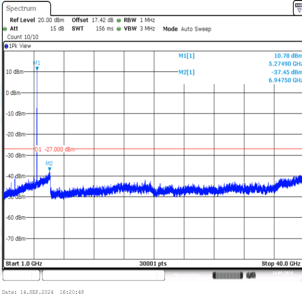
11N20MIMO-Ant1-5280-1000~40000-PASS
