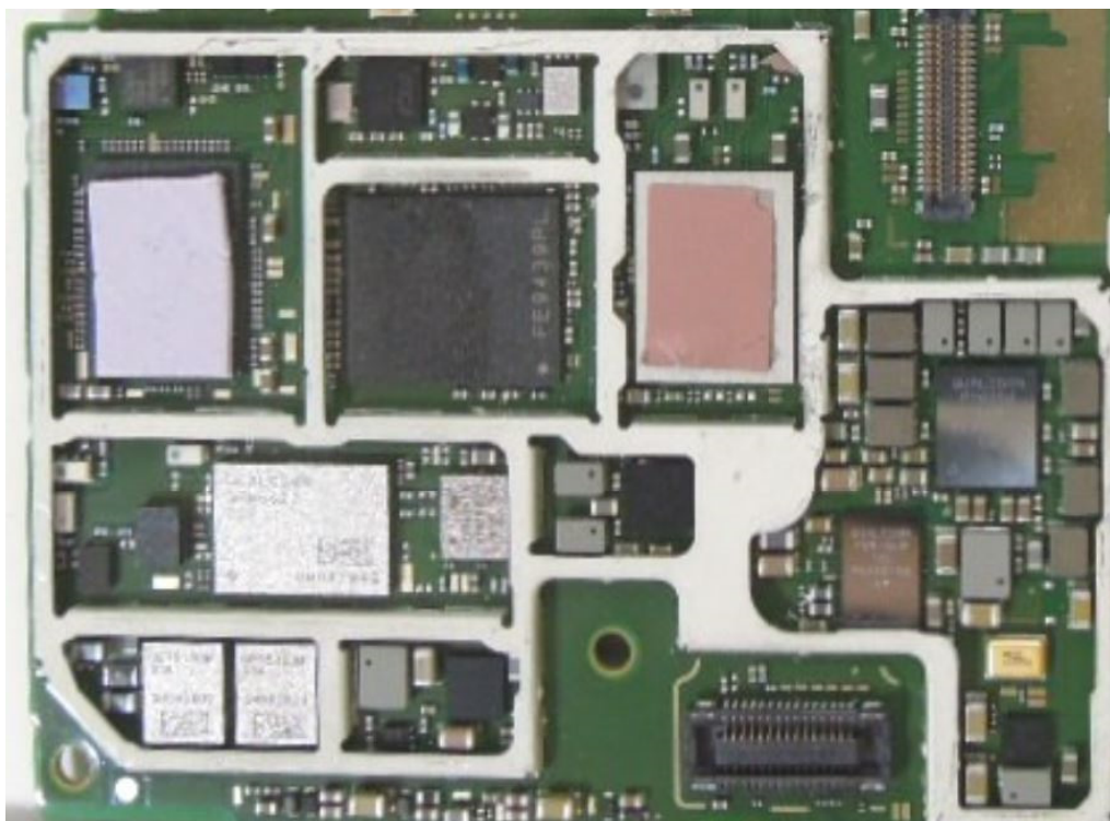
Internal View of EUT – 6
