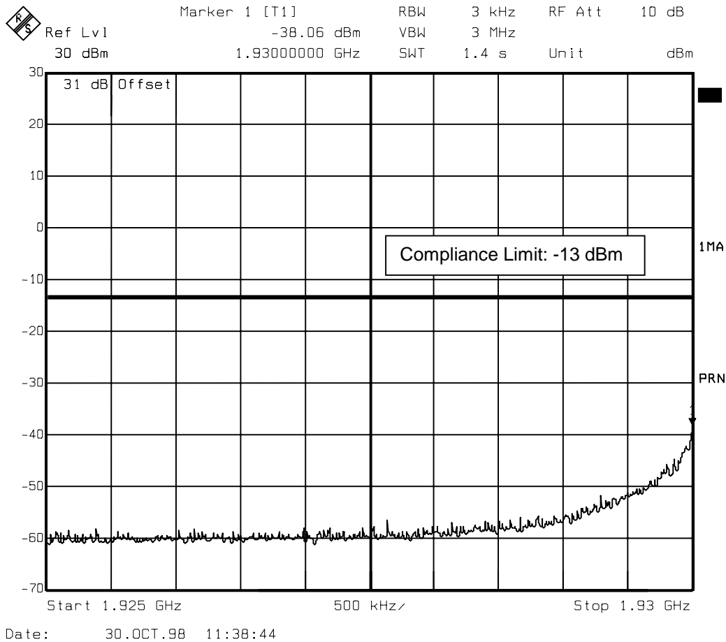
Fig. 10 – Spurious emissions in the frequency range 1925 MHz – 1930 MHz.
