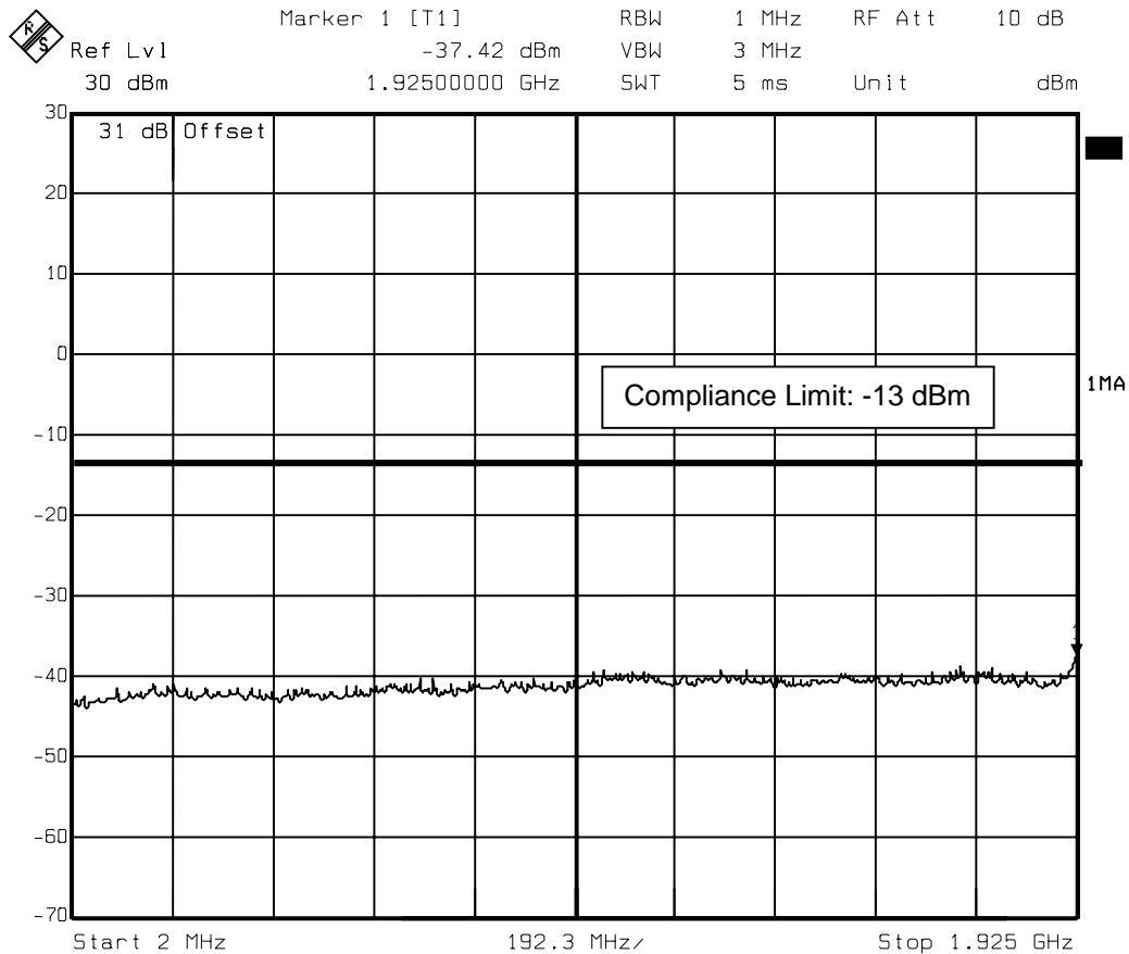
Fig. 19 – Spurious emissions in the frequency range 2 MHz – 1925 MHz.
