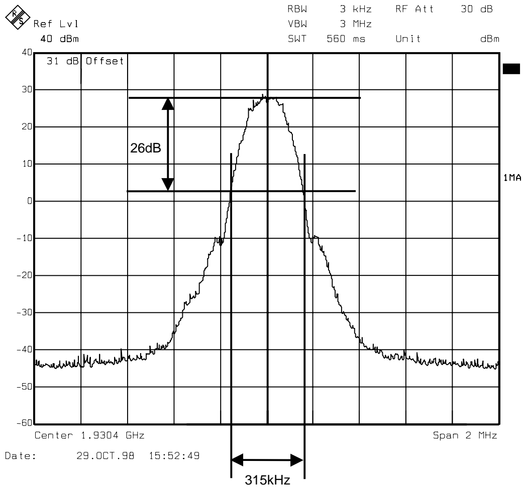
Fig. 6 – Occupied bandwidth.
