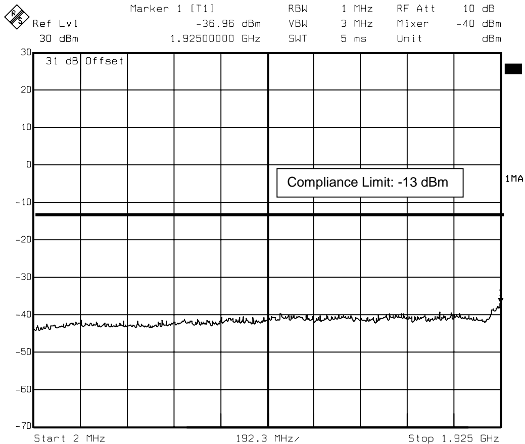
Fig. 14 – Spurious emissions in the frequency range 2 MHz – 1925 MHz.
