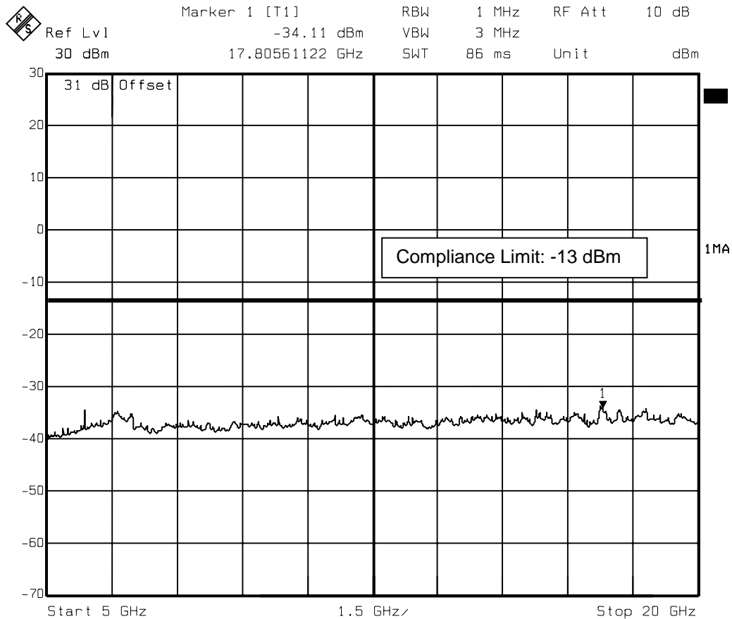
Fig. 18 – Spurious emissions in the frequency range 5000 MHz – 20000 MHz.
