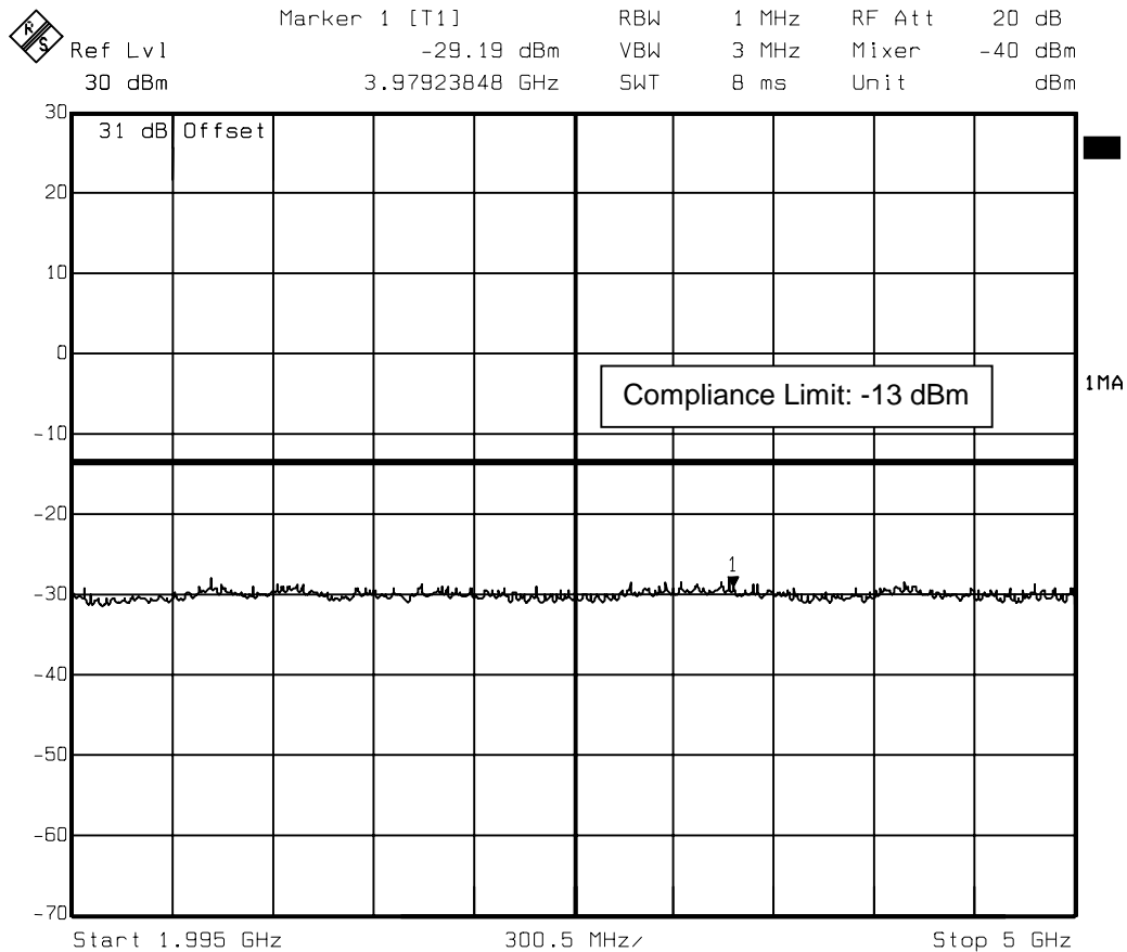
Fig. 22 – Spurious emissions in the frequency range 1995 MHz – 5000 MHz.
