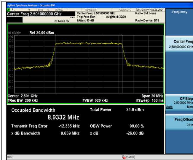
Band41-10MHz-QPSK-39700-50RB#0-PASS
