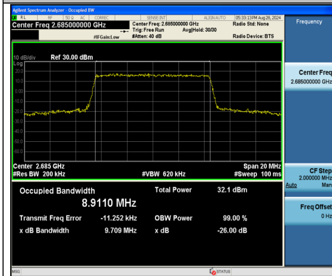
Band41-10MHz-QPSK-41540-50RB#0-PASS
