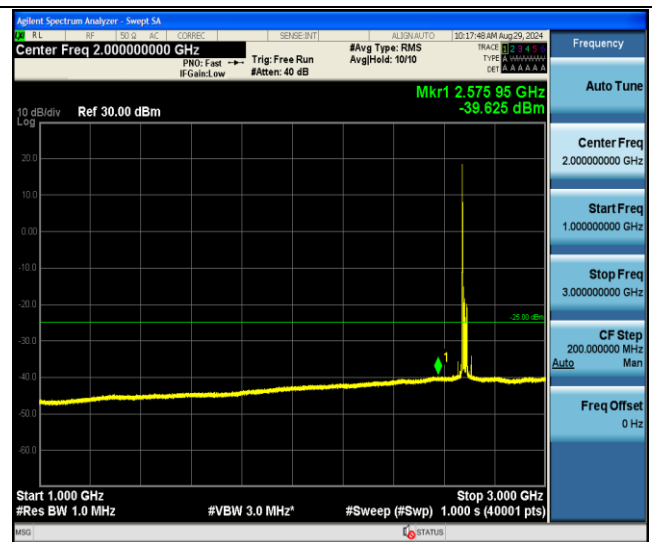
Band41-20MHz-QPSK-41490-1RB#0-1000~3000-PASS
