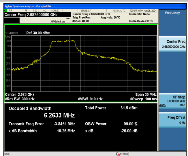
Band41-15MHz-16QAM-41515-27RB#0-PASS
