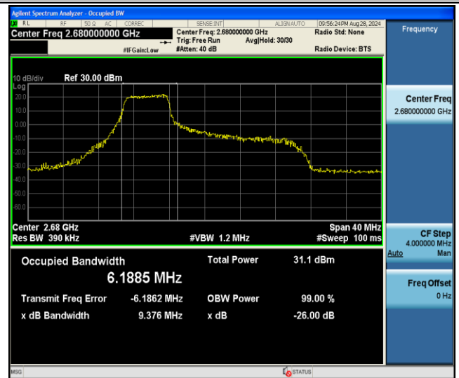
Band41-20MHz-16QAM-41490-27RB#0-PASS
