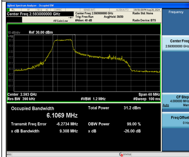
Band41-20MHz-16QAM-40620-27RB#0-PASS
