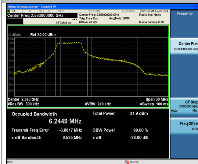
Band41-15MHz-16QAM-40620-27RB#0-PASS
