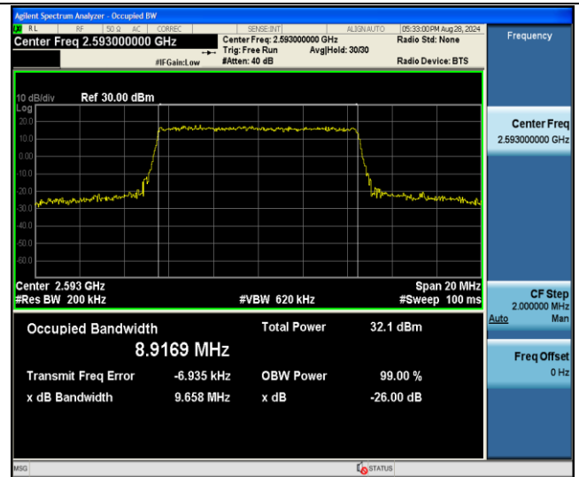
Band41-10MHz-QPSK-40620-50RB#0-PASS
