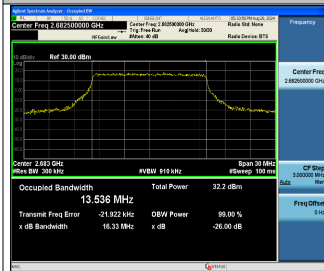
Band41-15MHz-QPSK-41515-75RB#0-PASS
