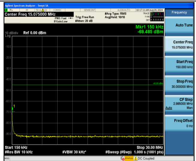
Band41-20MHz-QPSK-41490-1RB#0-0.15~30-PASS
