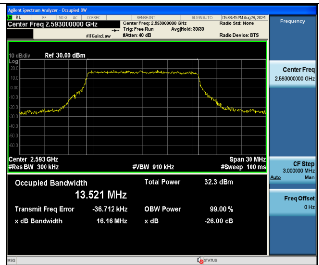
Band41-15MHz-QPSK-40620-75RB#0-PASS
