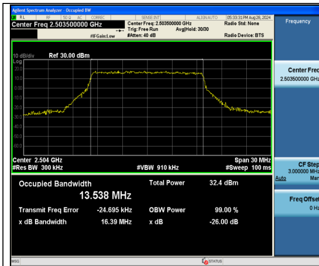
Band41-15MHz-QPSK-39725-75RB#0-PASS
