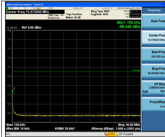
Band41-20MHz-QPSK-40620-1RB#0-0.15~30-PASS
