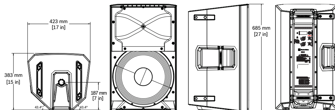
Figure 7.2: Dimensions ZLX-15BT
