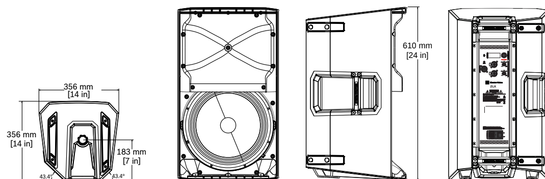
Figure 7.1: Dimensions ZLX-12BT
