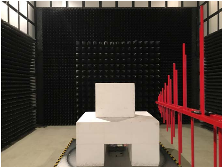
Part 22&24 RAD Front View (Below 1 GHz)
