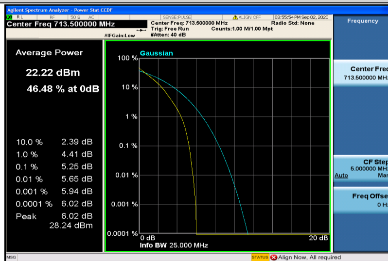
Band12-5MHz-QPSK-23155-25RB#0
