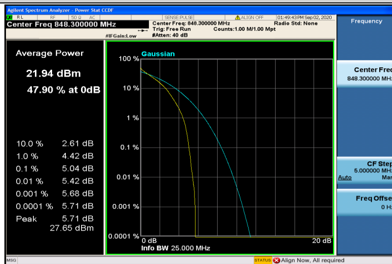
Band5-1.4MHz-QPSK-20643-6RB#0
