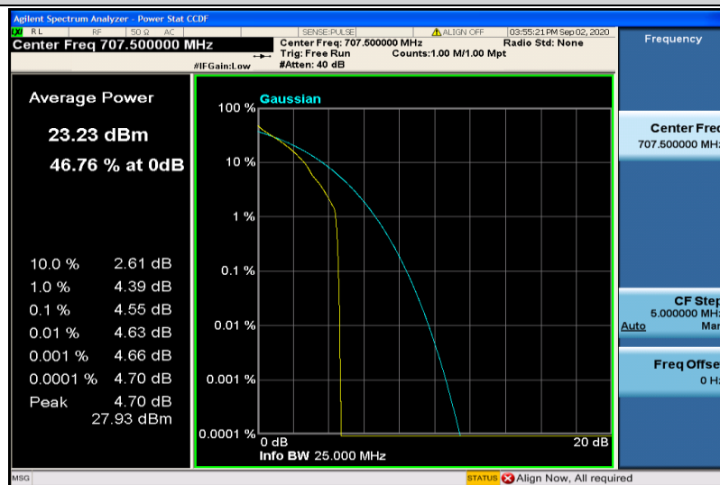
Band12-5MHz-QPSK-23095-1RB#0
