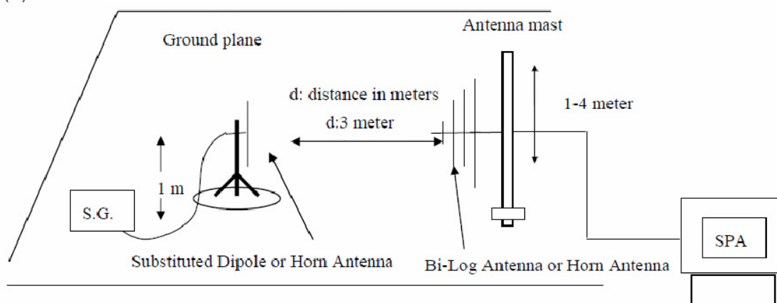
(C) Substituted Method Test Set-UP
