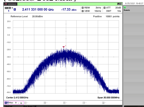
[ 802.11b/ 2412 MHz ]
