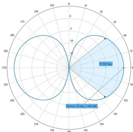
Elevation Pattern Referenced to +5dBi
