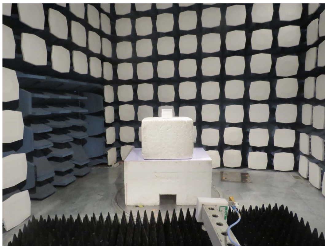
26.5GHz - 40GHz
