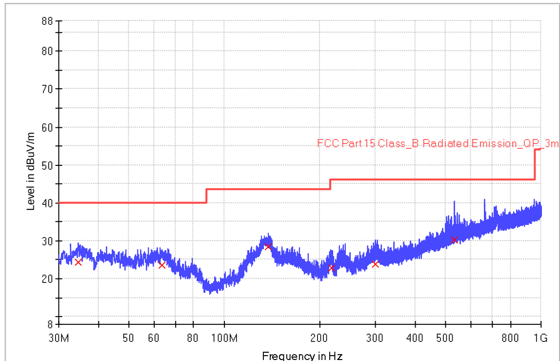
RE_VULB9168_pre_Cont_30-1000
