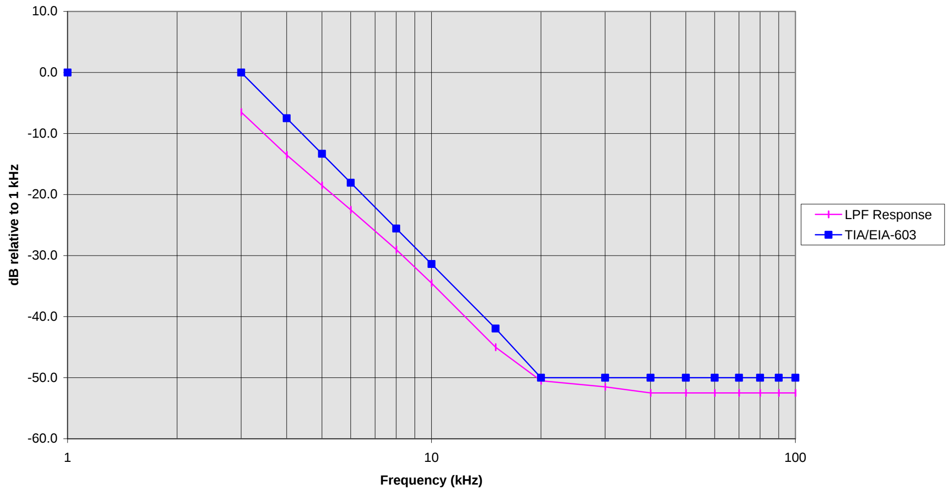
Audio Low Pass Filter Response
