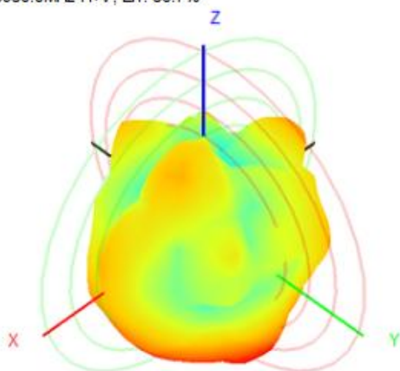
5850.0MHz H+V, Eff: 56.7%
