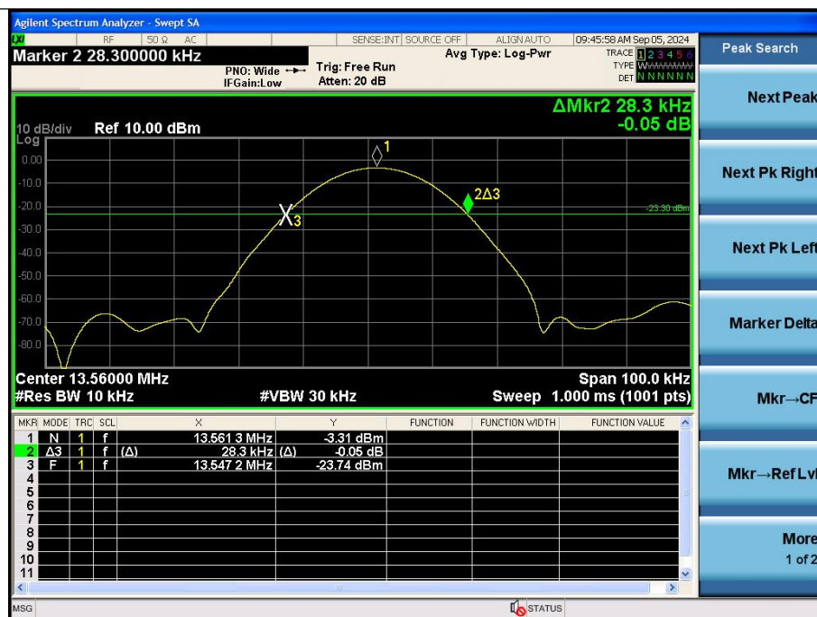
ASK Modulation
